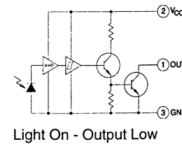
OPL801-OC (Open-Collector Output) Inverter
