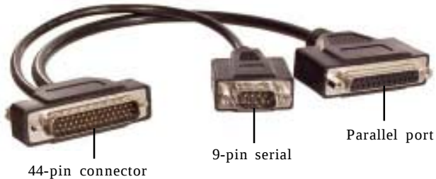
Figure 2. 1S1P fan-out cable
