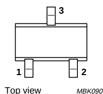
Fig.1 Simplified outline (SOT416).
