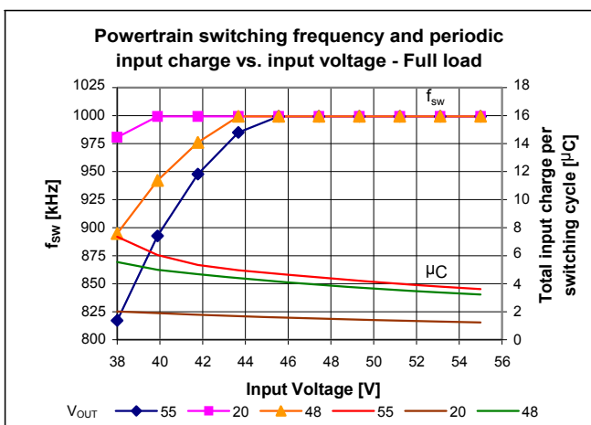
Figure 15 – Powertrain switching frequency and periodic input charge vs. V_{IN} , V_{OUT} ; I_{OUT} = 4.17 A
