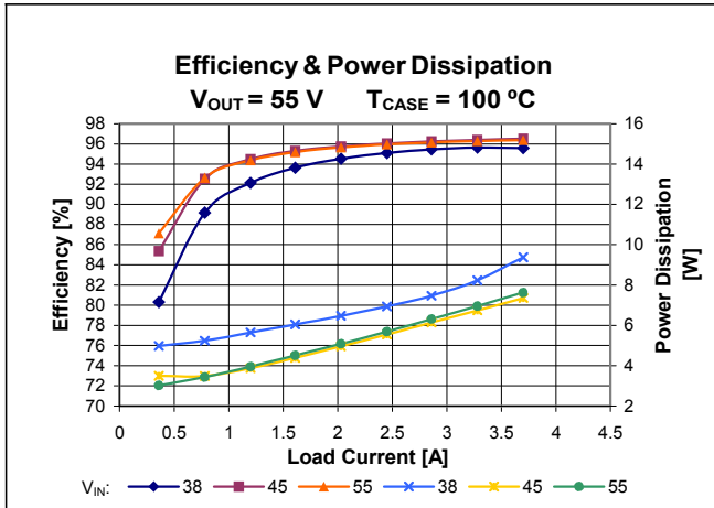
Figure 11 – Total efficiency and power dissipation vs. V_{IN} and I_{OUT} , V_{OUT} = 55 V, T_{CASE} = 100 °C
