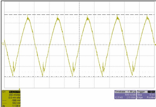
Figure 13 – Typical output voltage ripple waveform, T_{CASE} = 30 °C, V_{IN} = 45 V, V_{OUT} = 48 V, I_{OUT} = 4.17 A, no external capacitance.
