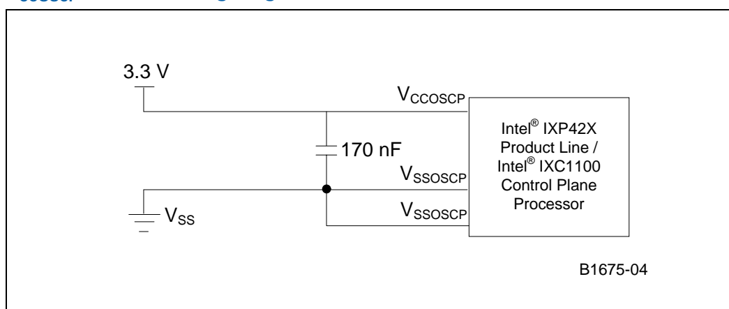
Figure 11. V_{CCOSC} Power Filtering Diagram
