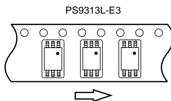
Outline and Dimensions (Reel)
