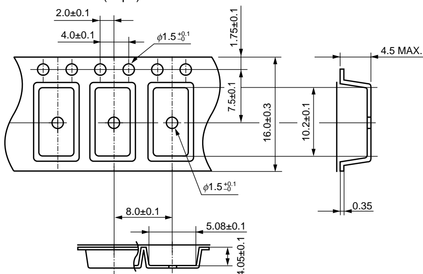
Outline and Dimensions (Tape)
