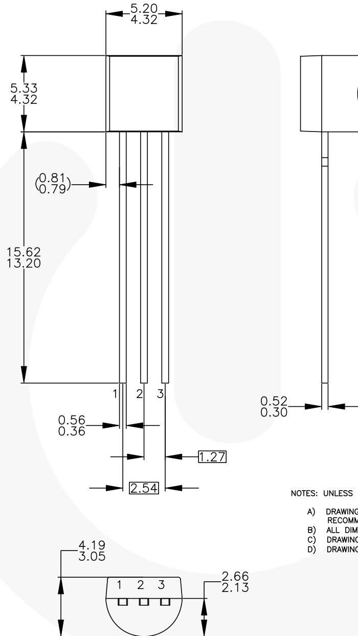
Figure 1. 3-Lead, TO-92, Molded, STD Straight Lead, Bulk Type
