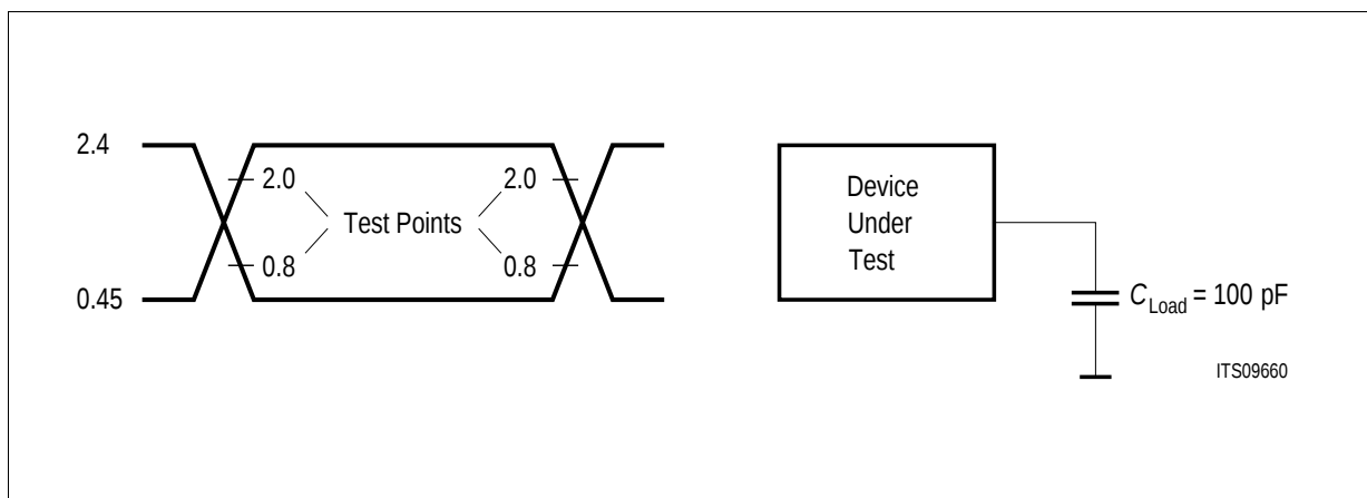
Figure 84 Input/Output Waveform for AC Tests
