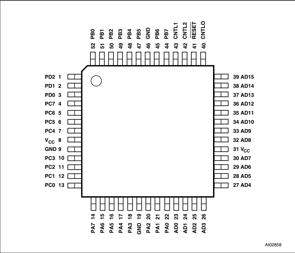
Figure 1. PQFP52 connections
