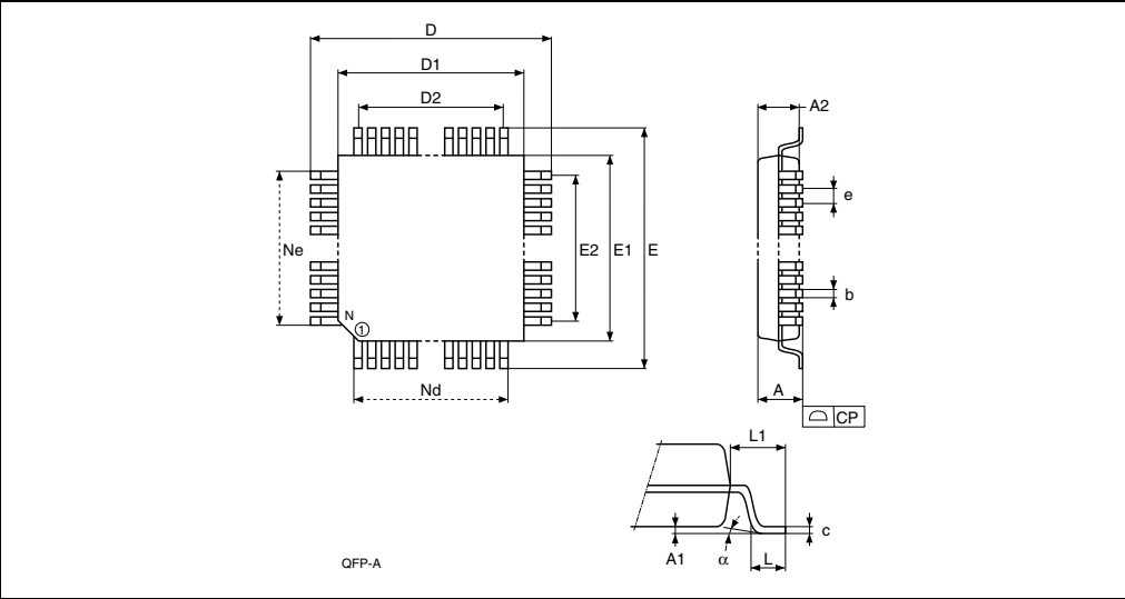
Figure 52. TQFP64 - 64-lead thin quad flatpack, package outline
