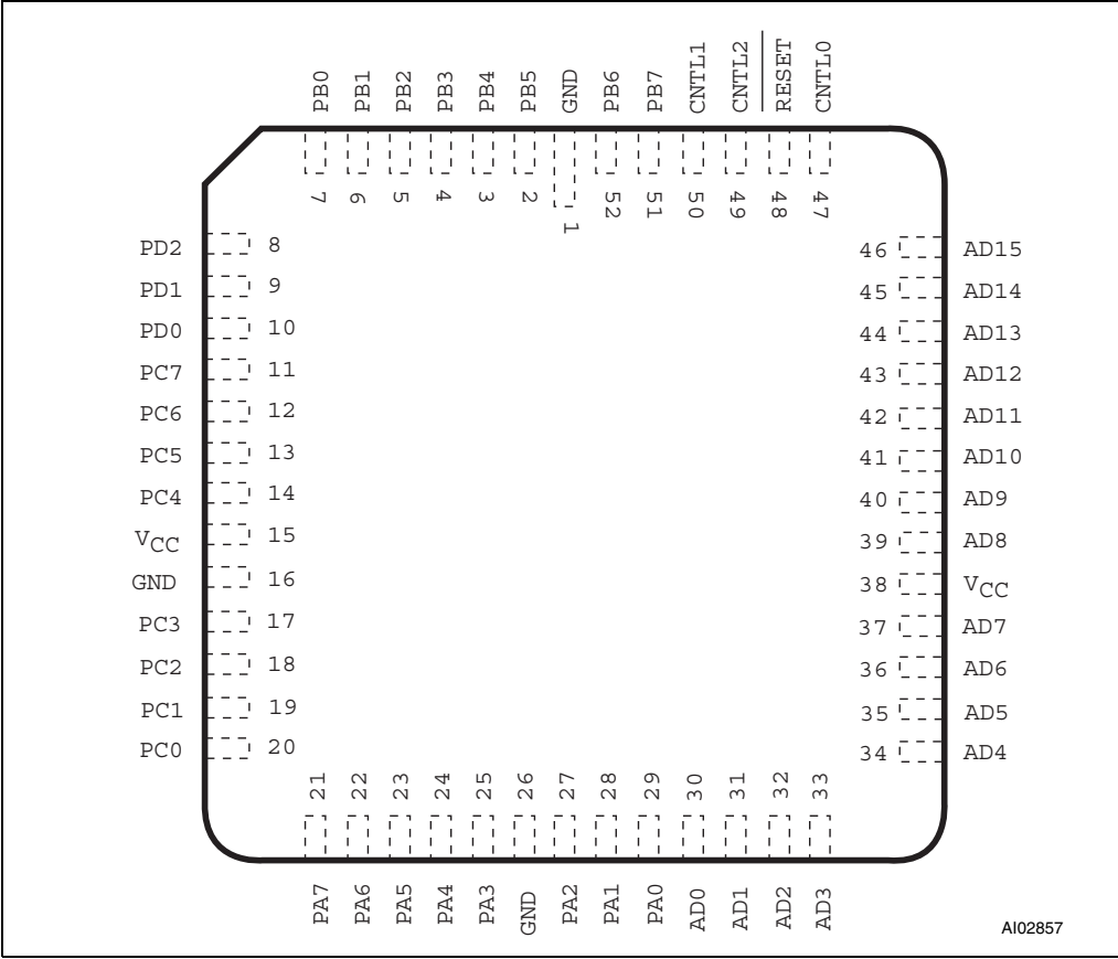
Figure 2. PLCC52 connections
