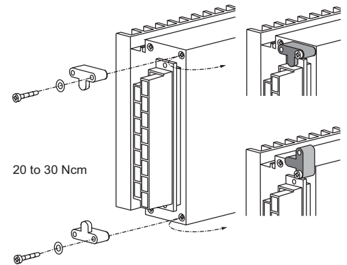
Fig. 22 Connector retention brackets HZZ01216-G
