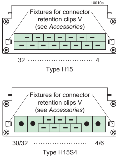
Fig. 17 View of H15 and H15S4 male connector
