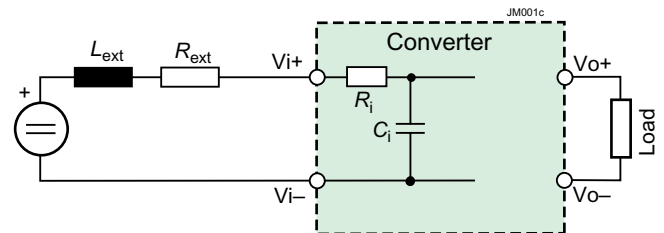
Fig. 2 Equivalent input circuit
