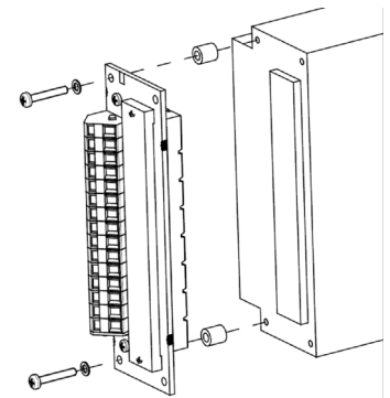
Fig. 23 Cage clamp adapter HZZ00144-G
