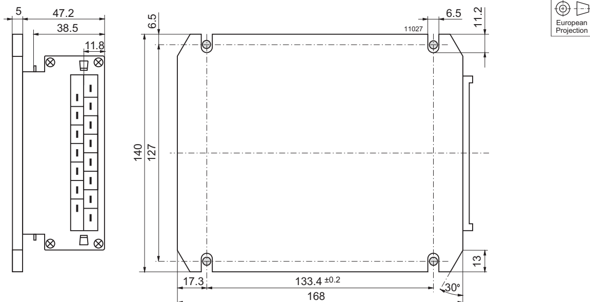
Fig. 15 Option B, large cooling plate Weight: 1.3 kg
