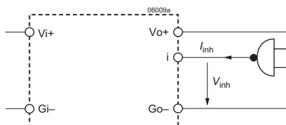
Fig. 6 Specification of the inhibit signal (typical)
