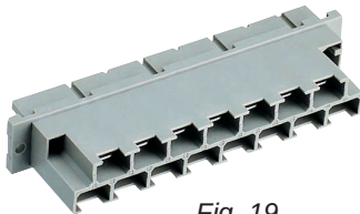
Fig. 19 H15 female connector with code key system
