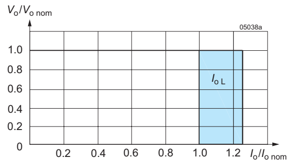
Fig. 4 Overload, short-circuit behavior V_o versus I_o .
