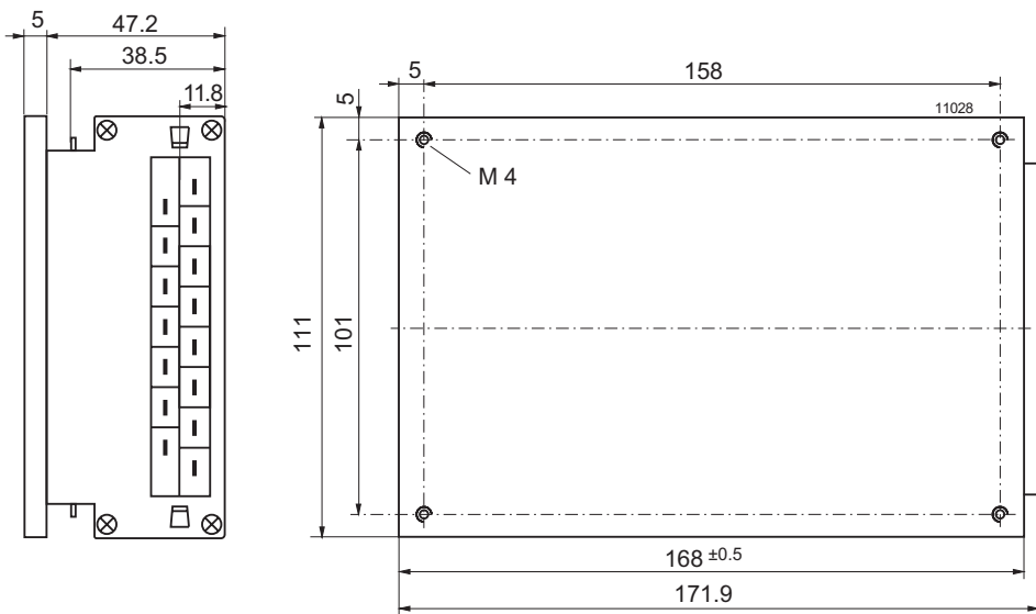
Fig. 16 Option B1, small cooling plate Weight: 1.2 kg
