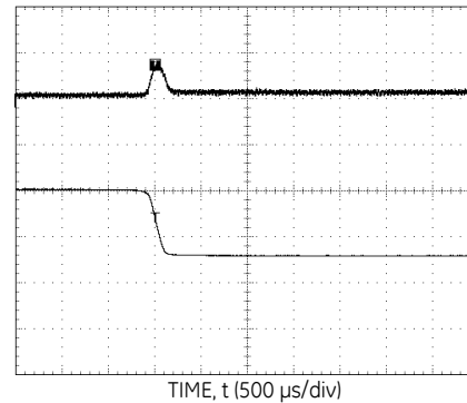
Figure 29. Typical Transient Response to Step change in Load from 50% to 25% of Full Load at Room Temperature and 48 Vdc Input.
