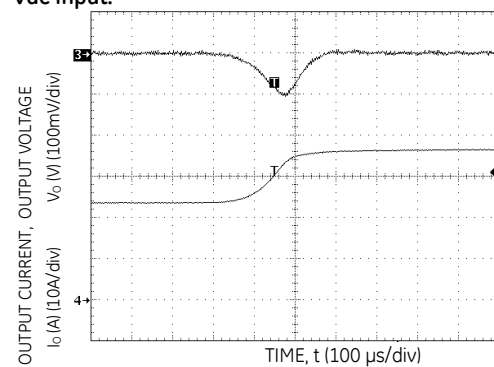
Figure 6. Typical Transient Response to Step change in Load from 50% to 75% of Full Load and 48 Vdc Input.
