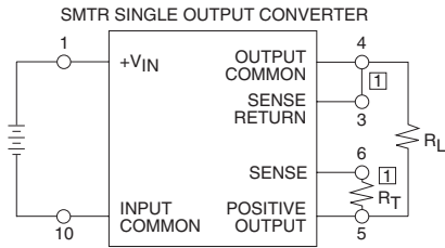
EXTERNAL TRIM CONNECTION ① Make connections at converter.
