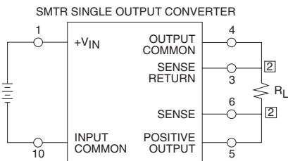
REMOTE SENSE CONNECTION ② Make connections at load.
