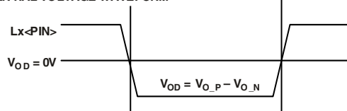
Figure 15. Link Ports—Signals Definition
