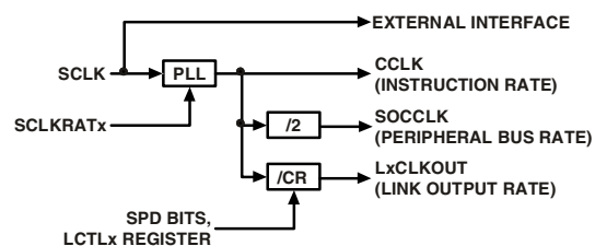
Figure 3. Clock Domains
