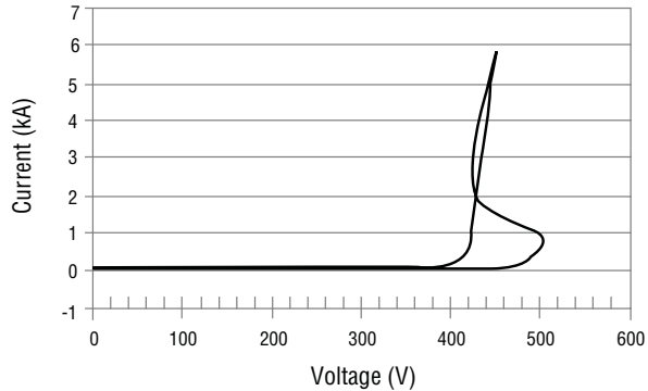
Surge Response - PTVS6-430C
