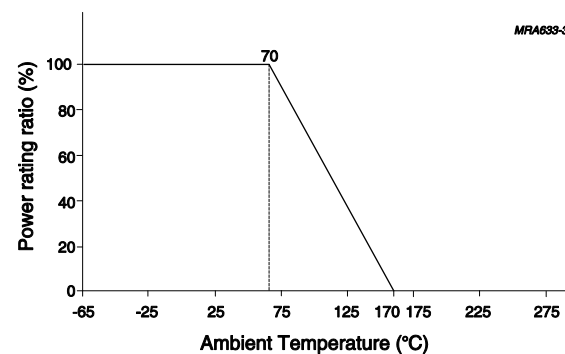
Fig. 4-2 Maximum dissipation ( P_{max} ) in percentage of rated power as a function of the operating ambient temperature ( T_{amb} )
