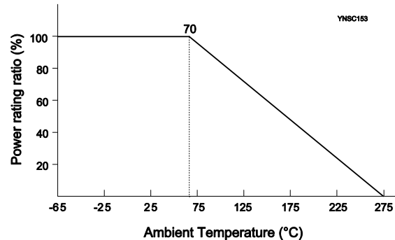
Fig. 4-1 Maximum dissipation ( P_{max} ) in percentage of rated power as a function of the operating ambient temperature ( T_{amb} )
