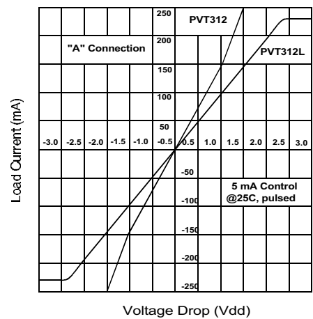
Figure 3. Linearity Characteristics
