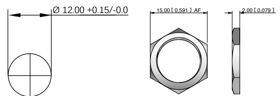
PANEL CUTOUT
