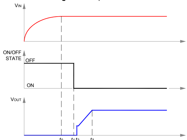
Fig. 8: Start-up scenario #2.
