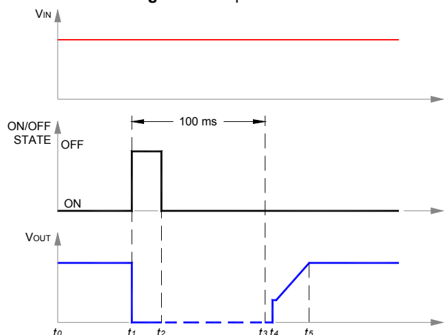
Fig. 9: Start-up scenario #3.
