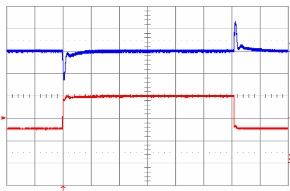
Fig. 21: Output voltage response to load current step-change (7.5 A – 15 A – 7.5 A) at V_{in} = 48 V. Top trace: output voltage (100 mV/div.). Bottom trace: load current (5 A/div.). Current slew rate: 5 A/ \mu s. C_o = 450 \mu F tantalum + 1 \mu F ceramic. Time scale: 0.2 ms/div.
