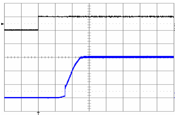
Fig. 19: Turn-on transient at full rated load current (resistive) plus 10,000 \mu F at V_{in} = 48 V, triggered via ON/OFF pin. Top trace: ON/OFF signal (5 V/div.). Bottom trace: output voltage (0.5 V/div.). Time scale: 1 ms/div.
