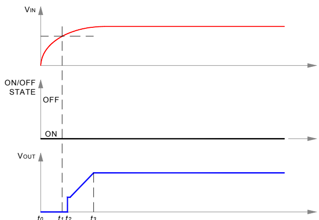
Fig. 7: Start-up scenario #1.
