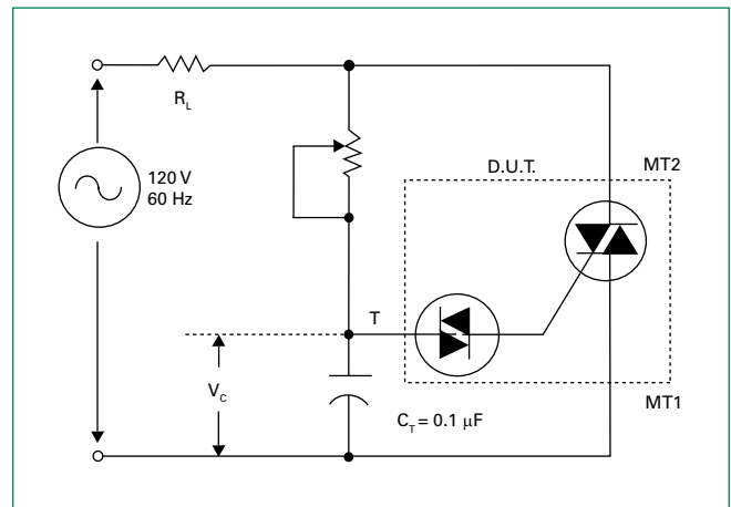
Figure 7: Test Circuit
