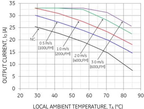
Figure 20. Output Current Derating for the Base plate QBW033A0B-H in the Transverse Orientation; Airflow Direction from Vin(-) to Vin(+); Vin = 48V.
