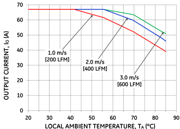
Figure 21. Output Current Derating for the Base plate QBVE067A0Bxx-H+1.0" Heat Sink in the Transverse Orientation; Airflow Direction from Vin(-) to Vin(+); Vin = 50V.
