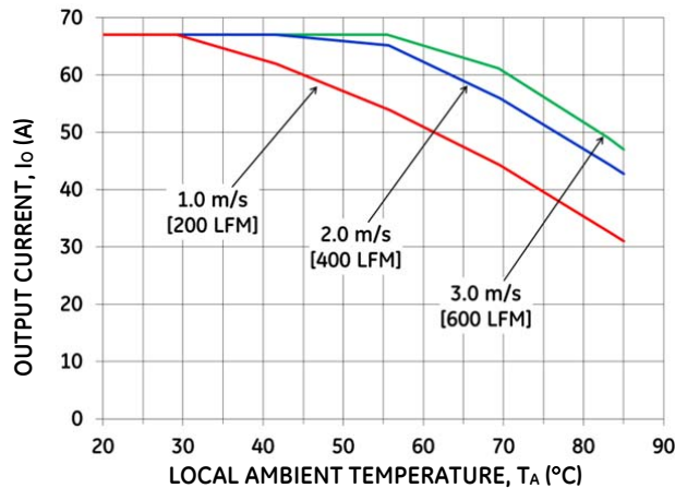
Figure 19. Output Current Derating for the Base plate QBVE067A0Bxx-H+0.5" Heat Sink in the Transverse Orientation; Airflow Direction from Vin(-) to Vin(+); Vin = 50V.
