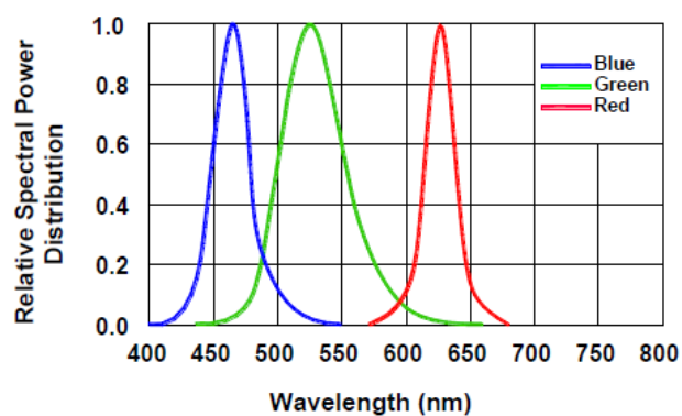
Figure 4. Relative Spectral Power Distribution vs. Wavelength
