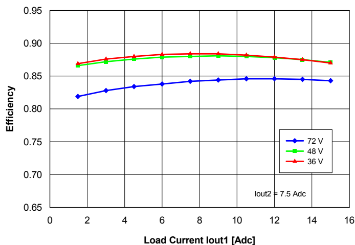
Fig. 17: Efficiency vs. load current Iout1 and input voltage for converter mounted horizontally with air flowing from pin 3 to pin 4 at a rate of 300 LFM (1.5 m/s), for Iout2 = 7.5 A and Ta = 25°C.
