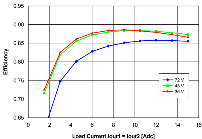
Fig. 21: Efficiency vs. balanced load current ( I_{out1} = I_{out2} ) and input voltage for converter mounted horizontally with air flowing from pin 3 to pin 4 at a rate of 300 LFM (1.5 m/s) and T_a = 25^\circ\text{C} .
