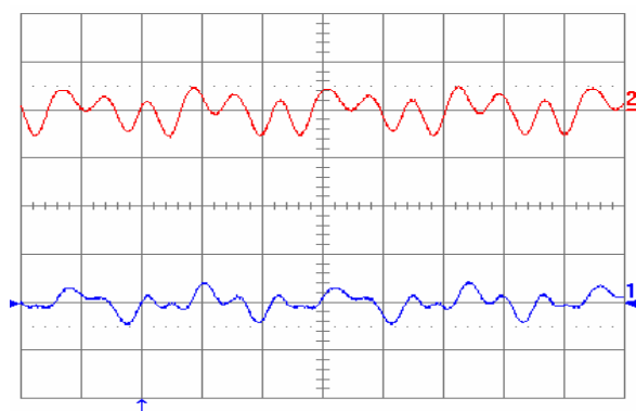
Fig. 34: Output voltage ripple at full rated load current into a resistive load on both outputs with Co = 1uF (ceramic) and Vin = 48 V. Ch2 = Vout2, Ch1 = Vout1 (both 20 mV/div). Time scale: 1 μs/div.
