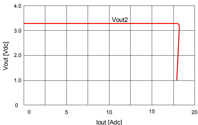
Fig. 31: Output voltage Vout2 vs. load current Iout2 showing current limit point and converter shutdown point. When Vout2 is in current limit, Vout1 will follow with less than 0.6 V difference until shut-down threshold of 1 V. Input voltage has almost no effect on Vout2 current limit characteristic.
