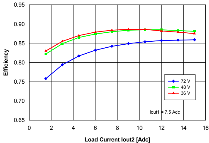
Fig. 19: Efficiency vs. load current Iout2 and input voltage for converter mounted horizontally with air flowing from pin 3 to pin 4 at a rate of 300 LFM (1.5 m/s), for Iout1 = 7.5 A and Ta = 25°C.
