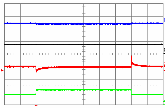
Fig. 27: Output voltage response to Iout2 load current step-change of 3.75 A (50%-75%-50%) at Iout1 = 7.5 A and Vin = 48 V. Ch1 = Vout1 (100 mV/div), Ch2 = Vout2 (100 mV/div), Ch3 = Iout1 (10 A/div.), Ch4 = Iout2 (10 A/div.). Current slew rate: 5 A/μs, Co = 300 μF tantalum + 1 μF ceramic. Time scale: 0.5 ms/div.
