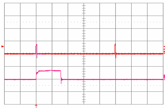
Fig. 33: Load current lout2 into a 10 mΩ short circuit on Vout2 during restart, with Vout1 open (no load), at Vin = 48 V. Ch2 = lout2 (20 A/div, 20 ms/div). ChB = lout2 (20 A/div, 1 ms/div) is an expansion of the on-time portion of lout2.
