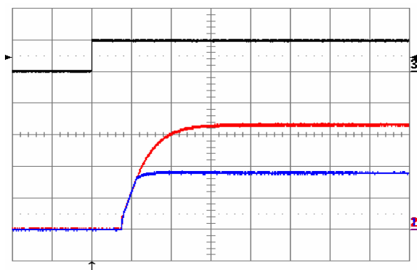
Fig. 22: Turn-on transient waveforms at no load current and V_{in} = 48\text{ V} , triggered via ON/OFF pin. Top trace: ON/OFF signal (5 V/div.). Bottom traces: V_{out1} (blue, 1 V/div.), V_{out2} (red, 1 V/div.). Time scale: 1 ms/div.
