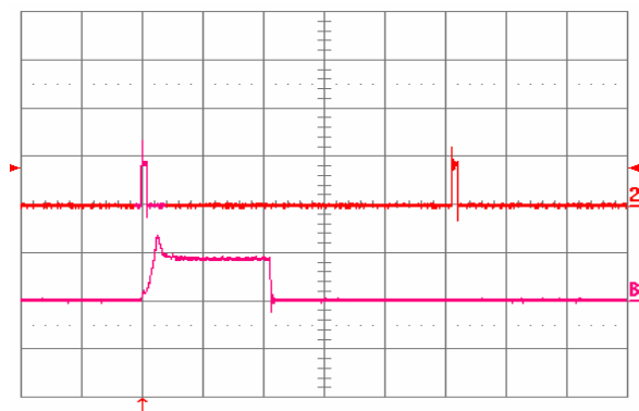
Fig. 32: Load current lout1 into a 10 mΩ short circuit on Vout1 during restart, with Vout2 open (no load), at Vin = 48 V. Ch2 = lout1 (20 A/div, 20 ms/div). ChB = lout1 (20 A/div, 1 ms/div) is an expansion of the on-time portion of lout1.
