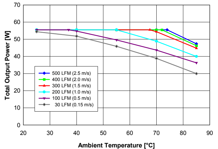
Fig. 9: Available output power for balanced load current ( I_{out1} = I_{out2} ) vs. ambient air temperature and airflow rates for converter with D height pins mounted horizontally with V_{in} = 48 V, air flowing from pin 3 to pin 1 and maximum FET temperature \leq 120^{\circ}\text{C} .
