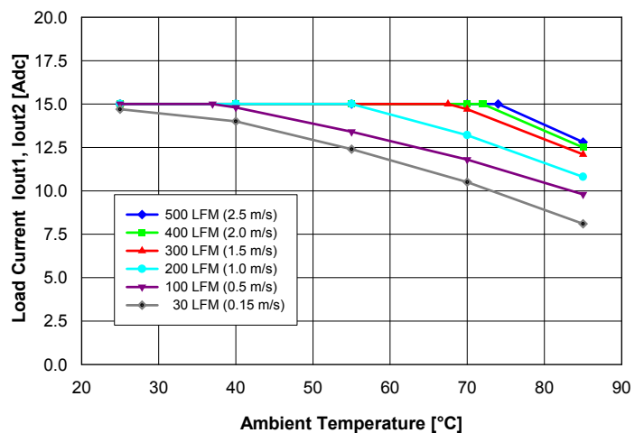
Fig. 11: Available balanced load current ( I_{out1} = I_{out2} ) vs. ambient air temperature and airflow rates for converter mounted with D height pins horizontally with V_{in} = 48 V, air flowing from pin 3 to pin 1 and maximum FET temperature \leq 120^{\circ}\text{C} .
