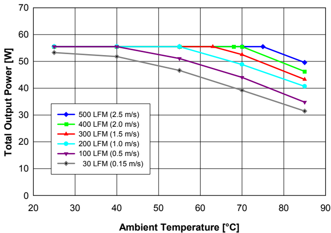
Fig. 8: Available output power for balanced load current ( I_{out1} = I_{out2} ) vs. ambient air temperature and airflow rates for converter with D height pins mounted vertically with V_{in} = 48 V, air flowing from pin 3 to pin 1 and maximum FET temperature \leq 120^{\circ}\text{C} .
