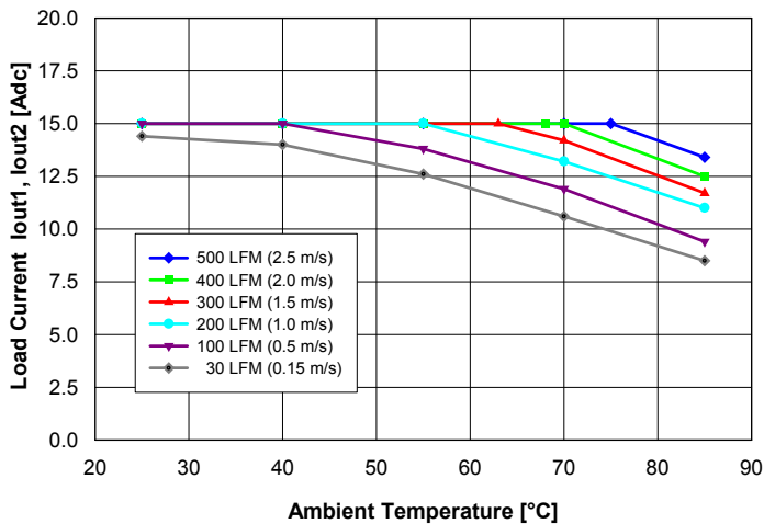
Fig. 10: Available balanced load current ( I_{out1} = I_{out2} ) vs. ambient air temperature and airflow rates for converter with D height pins mounted vertically with V_{in} = 48 V, air flowing from pin 3 to pin 1 and maximum FET temperature \leq 120^{\circ}\text{C} .
