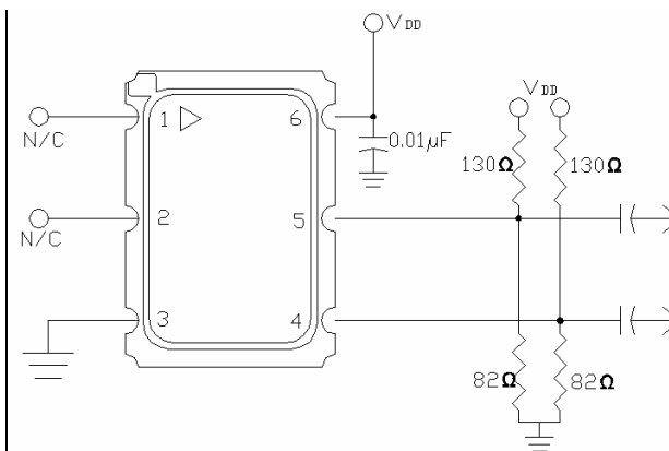
Figure 7. Pull-up Pull-down Termination
