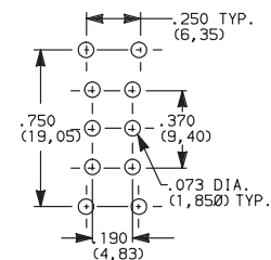
PC MOUNTING
