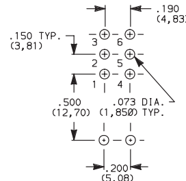
PC MOUNTING
