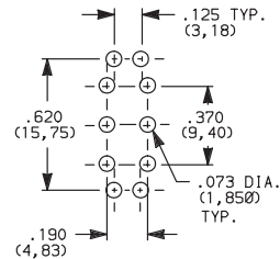
8261SH9_BE2 DPDT
