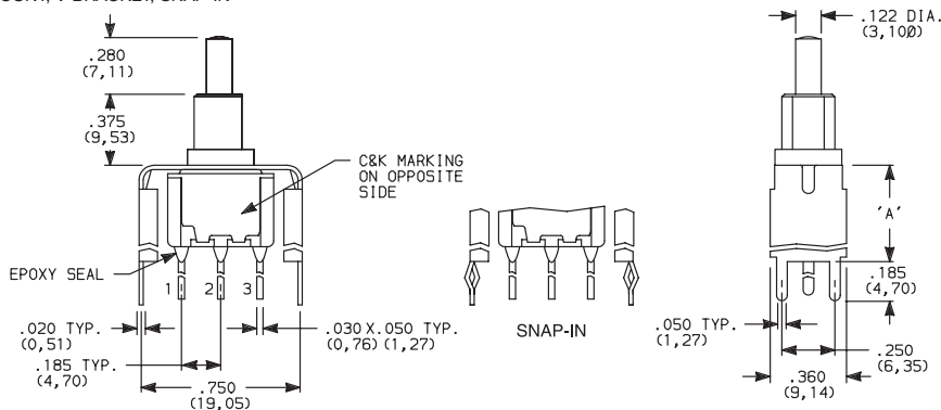
8161SH9_BE2 SPDT
