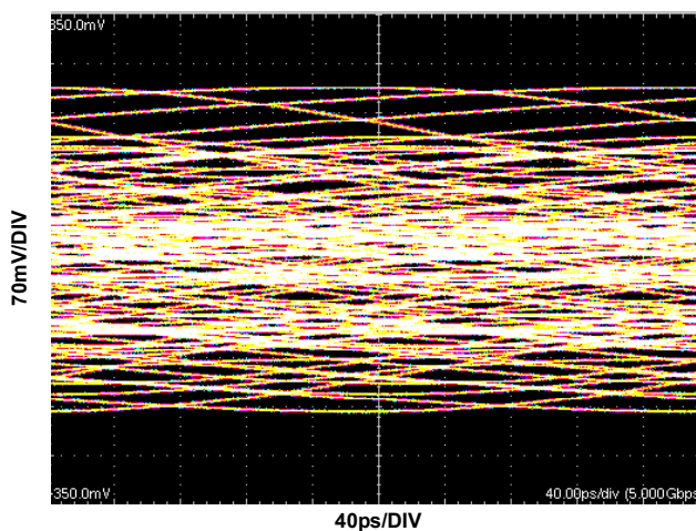
FIGURE 9. RECEIVED SIGNAL AFTER 20m OF 28AWG TWIN-AXIAL CABLE (CABLE C) (Note 18), 5Gb/s
