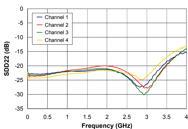
FIGURE 20. OUTPUT DIFFERENTIAL RETURN LOSS
