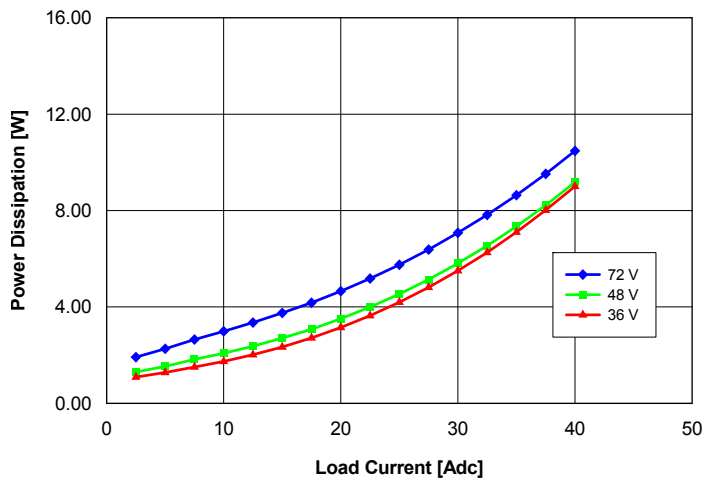
Fig. 1.0V.5: Power dissipation vs. load current and input voltage for converter mounted vertically with air flowing from pin 3 to pin 1 at a rate of 300 LFM (1.5 m/s) and T_a = 25^\circ\text{C} .
