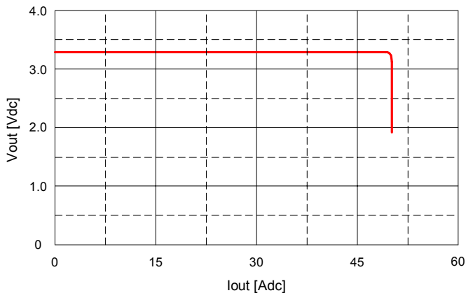
Fig. 3.3V.13: Output voltage vs. load current showing current limit point and converter shutdown point. Input voltage has almost no effect on current limit characteristic.
