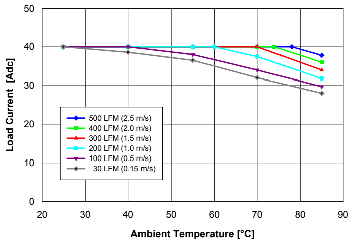
Fig. 1.0V.1: Available load current vs. ambient air temperature and airflow rates for QM48S40010 converter mounted vertically with air flowing from pin 3 to pin 1, MOSFET temperature \leq 120^{\circ}\text{C} , V_{in} = 48\text{ V} .
