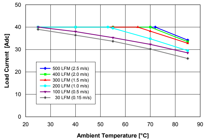
Fig. 1.5V.2: Available load current vs. ambient air temperature and airflow rates for QM48S40015 converter mounted horizontally with air flowing from pin 3 to pin 1, MOSFET temperature \leq 120^{\circ}\text{C} , V_{in} = 48\text{ V} .
