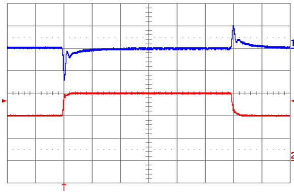
Fig. 1.0V.9: Output voltage response to load current step-change (20 A – 30 A – 20 A) at V_{in} = 48 V. Top trace: output voltage (100 mV/div.). Bottom trace: load current (10 A/div.). Current slew rate: 1 A/ \mu s. C_o = 470 \mu F tantalum + 1 \mu F ceramic. Time scale: 0.2 ms/div.
