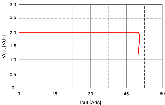
Fig. 2.0V.13: Output voltage vs. load current showing current limit point and converter shutdown point. Input voltage has almost no effect on current limit characteristic.
