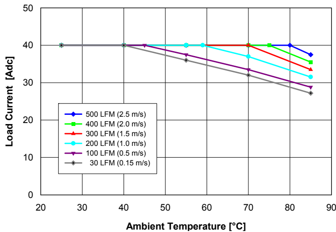
Fig. 1.2V.1: Available load current vs. ambient air temperature and airflow rates for QM48S40012 converter mounted vertically with air flowing from pin 3 to pin 1, MOSFET temperature \leq 120^{\circ}\text{C} , V_{in} = 48\text{ V} .
