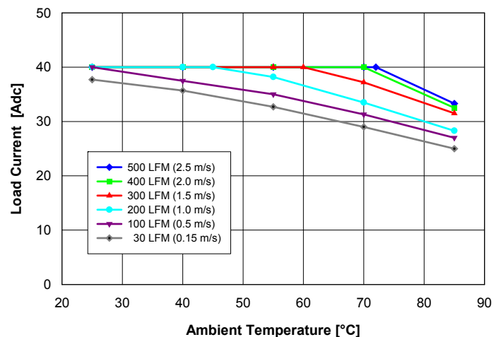
Fig. 1.8V.2: Available load current vs. ambient air temperature and airflow rates for QM48S40018 converter mounted horizontally with air flowing from pin 3 to pin 1, MOSFET temperature \leq 120^{\circ}\text{C} , V_{in} = 48\text{ V} .
