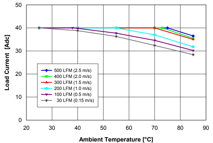
Fig. 1.0V.2: Available load current vs. ambient air temperature and airflow rates for QM48S40010 converter mounted horizontally with air flowing from pin 3 to pin 1, MOSFET temperature \leq 120^{\circ}\text{C} , V_{in} = 48\text{ V} .
