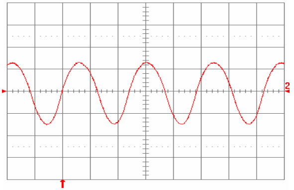
Fig. 2.0V.14: Input reflected ripple current, i_c (100 mA/div), measured at input terminals at full rated load current and V_{in} = 48 V. Refer to Fig. 2.0V.11 for test setup. Time scale: 1 \mu s/div.
