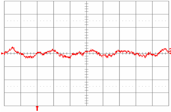
Fig. 1.8V.12: Input reflected ripple current, i_s (10 mA/div), measured through 10 \mu H at the source at full rated load current and V_{in} = 48 V. Refer to Fig. 1.8V.11 for test setup. Time scale: 1 \mu s/div.
