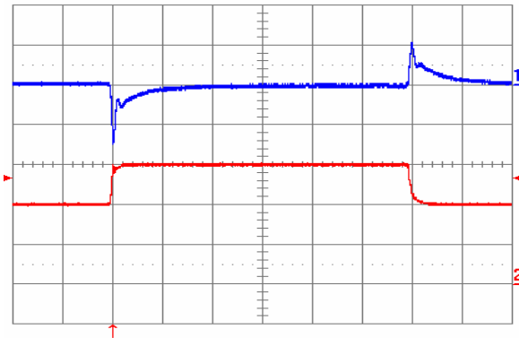
Fig. 1.5V.9: Output voltage response to load current step-change (20 A – 30 A – 20 A) at V_{in} = 48\text{ V} . Top trace: output voltage (100 mV/div.). Bottom trace: load current (10 A/div.). Current slew rate: 1 A/ \mu\text{s} . C_o = 470\text{ }\mu\text{F} tantalum + 1 \mu\text{F} ceramic. Time scale: 0.2 ms/div.
