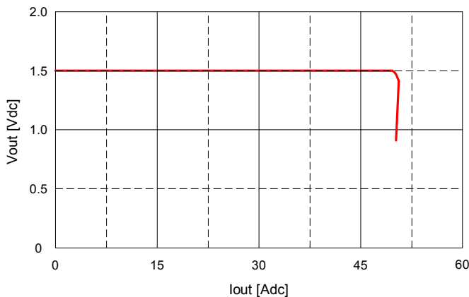
Fig. 1.5V.13: Output voltage vs. load current showing current limit point and converter shutdown point. Input voltage has almost no effect on current limit characteristic.
