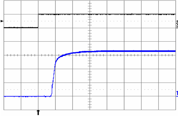
Fig. 3.3V.7: Turn-on transient at full rated load current (resistive) with no output capacitor at V_{in} = 48\text{ V} , triggered via ON/OFF pin. Top trace: ON/OFF signal (5 V/div.). Bottom trace: output voltage (1 V/div.). Time scale: 2 ms/div.
