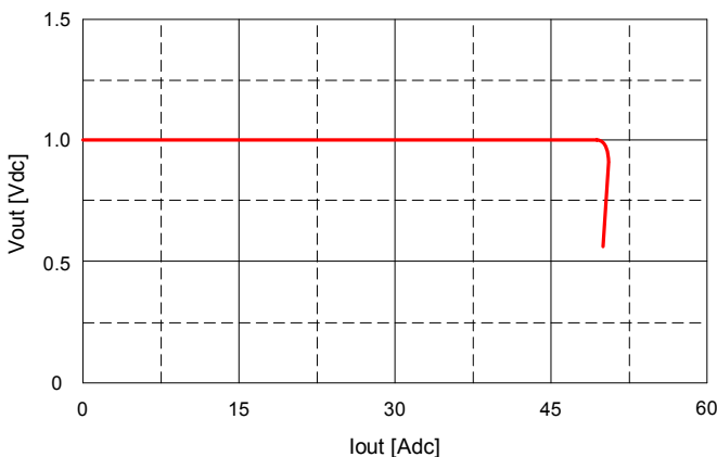
Fig. 1.0V.13: Output voltage vs. load current showing current limit point and converter shutdown point. Input voltage has almost no effect on current limit characteristic.
