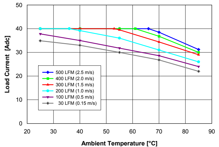
Fig. 2.5V.2: Available load current vs. ambient air temperature and airflow rates for QM48S40025 converter mounted horizontally with air flowing from pin 3 to pin 1, MOSFET temperature \leq 120^{\circ}\text{C} , V_{in} = 48\text{ V} .
