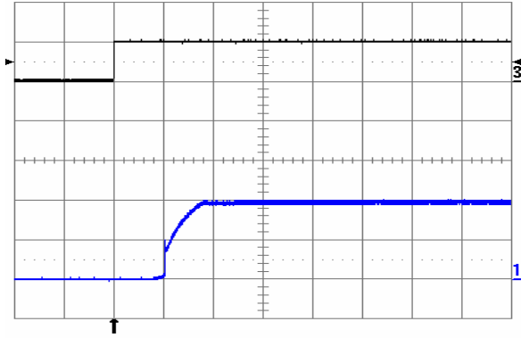
Fig. 1.0V.8: Turn-on transient at full rated load current (resistive) plus 40,000 \mu F at V_{in} = 48 V, triggered via ON/OFF pin. Top trace: ON/OFF signal (5 V/div.). Bottom trace: output voltage (0.5 V/div.). Time scale: 2 ms/div.
