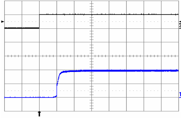
Fig. 1.0V.7: Turn-on transient at full rated load current (resistive) with no output capacitor at V_{in} = 48 V, triggered via ON/OFF pin. Top trace: ON/OFF signal (5 V/div.). Bottom trace: output voltage (0.5 V/div.). Time scale: 2 ms/div.
