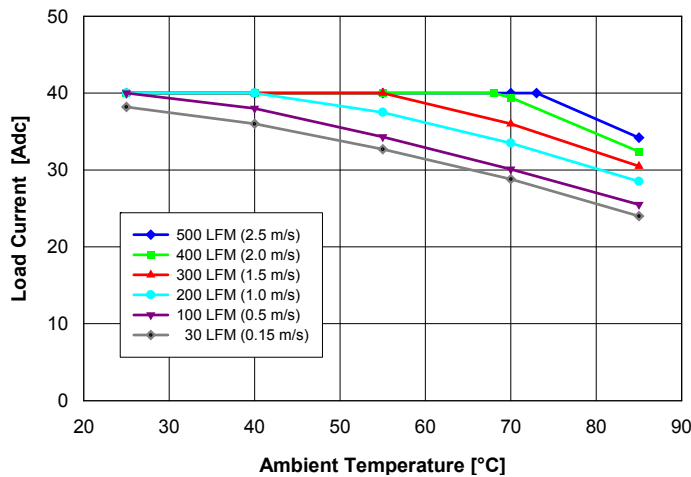
Fig. 2.0V.1: Available load current vs. ambient air temperature and airflow rates for QM48S40020 converter mounted vertically with air flowing from pin 3 to pin 1, MOSFET temperature \leq 120^{\circ}\text{C} , V_{in} = 48\text{ V} .
