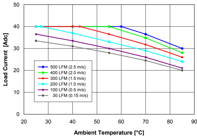
Fig. 3.3V.1: Available load current vs. ambient air temperature and airflow rates for QM48S40033 converter mounted vertically with air flowing from pin 3 to pin 1, MOSFET temperature \leq 120^{\circ}\text{C} , V_{in} = 48\text{ V} .
