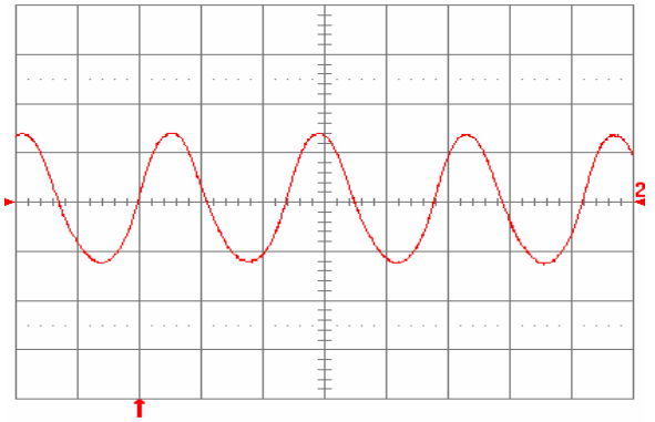
Fig. 3.3V.14: Input reflected ripple current, i_c (100 mA/div), measured at input terminals at full rated load current and V_{in} = 48 V. Refer to Fig. 3.3V.11 for test setup. Time scale: 1 \mu s/div.
