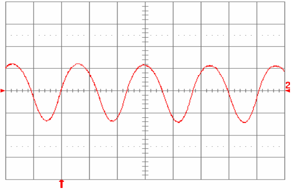
Fig. 1.8V.14: Input reflected ripple current, i_c (100 mA/div), measured at input terminals at full rated load current and V_{in} = 48 V. Refer to Fig. 1.8V.11 for test setup. Time scale: 1 \mu s/div.
