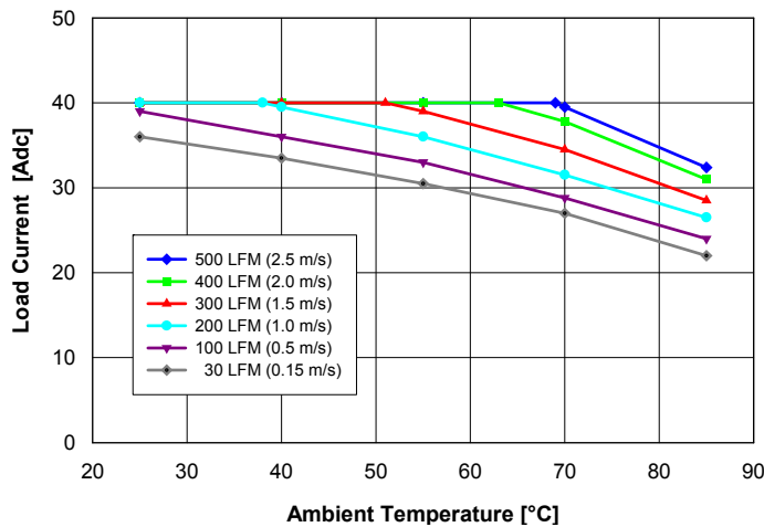
Fig. 2.5V.1: Available load current vs. ambient air temperature and airflow rates for QM48S40025 converter mounted vertically with air flowing from pin 3 to pin 1, MOSFET temperature \leq 120^{\circ}\text{C} , V_{in} = 48\text{ V} .
