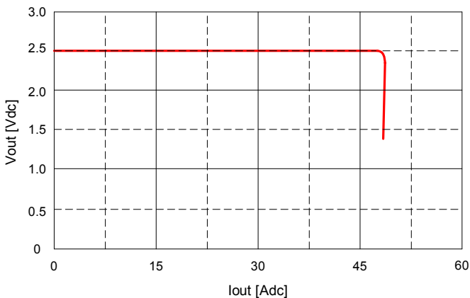
Fig. 2.5V.13: Output voltage vs. load current showing current limit point and converter shutdown point. Input voltage has almost no effect on current limit characteristic.
