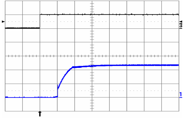
Fig. 1.2V.8: Turn-on transient at full rated load current (resistive) plus 40,000 \mu F at V_{in} = 48 V, triggered via ON/OFF pin. Top trace: ON/OFF signal (5 V/div.). Bottom trace: output voltage (0.5 V/div.). Time scale: 2 ms/div.
