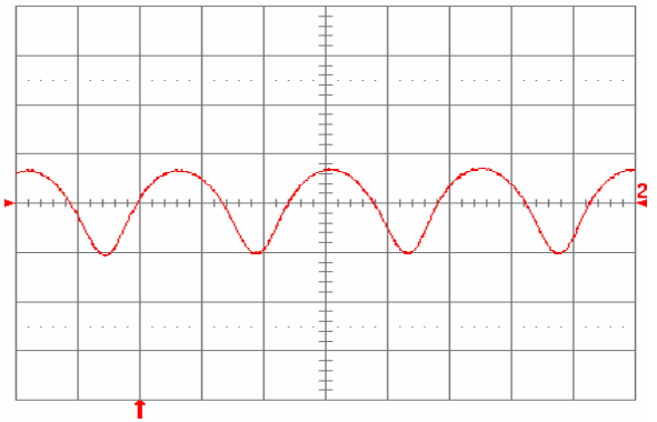
Fig. 1.0V.14: Input reflected ripple current, i_c (100 mA/div), measured at input terminals at full rated load current and V_{in} = 48 V. Refer to Fig. 1.0V.11 for test setup. Time scale: 1 \mu s/div.
