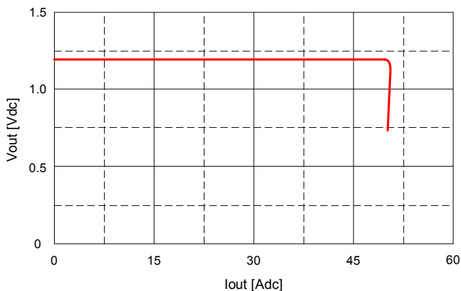
Fig. 1.2V.13: Output voltage vs. load current showing current limit point and converter shutdown point. Input voltage has almost no effect on current limit characteristic.
