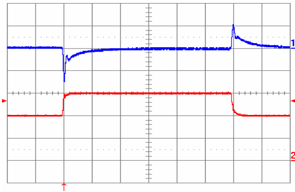
Fig. 1.8V.9: Output voltage response to load current step-change (20 A – 30 A – 20 A) at V_{in} = 48 V. Top trace: output voltage (100 mV/div.). Bottom trace: load current (10 A/div.). Current slew rate: 1 A/ \mu s. C_o = 470 \mu F tantalum + 1 \mu F ceramic. Time scale: 0.2 ms/div.
