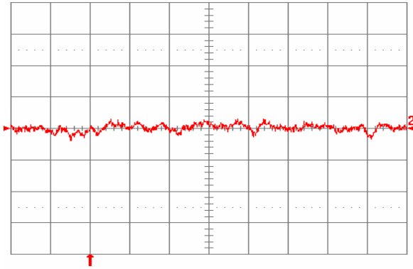
Fig. 1.5V.12: Input reflected ripple current, i_s (10 mA/div), measured through 10 \mu H at the source at full rated load current and V_{in} = 48 V. Refer to Fig. 1.5V.11 for test setup. Time scale: 1 \mu s/div.
