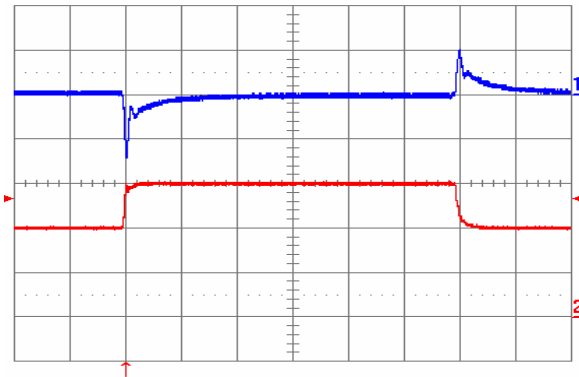
Fig. 2.5V.9: Output voltage response to load current step-change (20 A – 30 A – 20 A) at V_{in} = 48\text{ V} . Top trace: output voltage (100 mV/div.). Bottom trace: load current (10 A/div.). Current slew rate: 1 A/ \mu\text{s} . C_o = 470\text{ }\mu\text{F} tantalum + 1 \mu\text{F} ceramic. Time scale: 0.2 ms/div.
