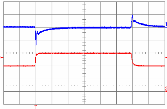
Fig. 3.3V.9: Output voltage response to load current step-change (20 A – 30 A – 20 A) at V_{in} = 48\text{ V} . Top trace: output voltage (100 mV/div.). Bottom trace: load current (10 A/div.). Current slew rate: 1 A/ \mu\text{s} . C_o = 470\text{ }\mu\text{F} tantalum + 1 \mu\text{F} ceramic. Time scale: 0.2 ms/div.
