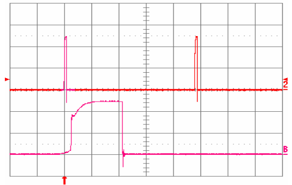
Fig. 2.5V.15: Load current (top trace, 20 A/div, 20 ms/div) into a 10 m \Omega short circuit during restart, at V_{in} = 48 V. Bottom trace (20 A/div, 1 ms/div) is an expansion of the on-time portion of the top trace.
