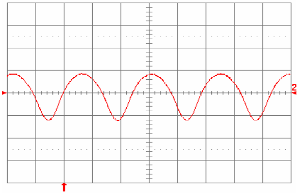
Fig. 1.2V.14: Input reflected ripple current, i_c (100 mA/div), measured at input terminals at full rated load current and V_{in} = 48 V. Refer to Fig. 1.2V.11 for test setup. Time scale: 1 \mu s/div.
