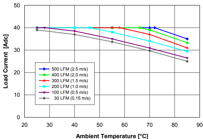
Fig. 1.8V.1: Available load current vs. ambient air temperature and airflow rates for QM48S40018 converter mounted vertically with air flowing from pin 3 to pin 1, MOSFET temperature \leq 120^{\circ}\text{C} , V_{in} = 48\text{ V} .
