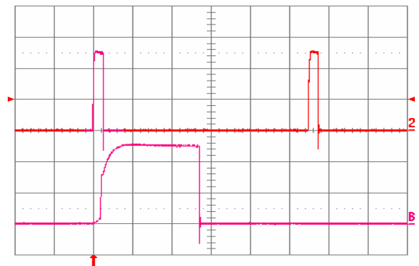
Fig. 1.8V.15: Load current (top trace, 20 A/div, 20 ms/div) into a 10 \Omega short circuit during restart, at V_{in} = 48 V. Bottom trace (20 A/div, 2 ms/div) is an expansion of the on-time portion of the top trace.
