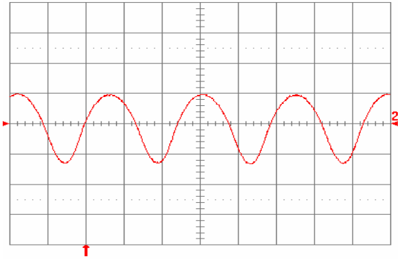
Fig. 1.5V.14: Input reflected ripple current, i_c (100 mA/div), measured at input terminals at full rated load current and V_{in} = 48 V. Refer to Fig. 1.5V.11 for test setup. Time scale: 1 \mu s/div.
