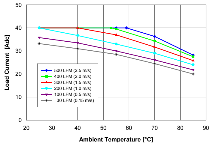
Fig. 3.3V.2: Available load current vs. ambient air temperature and airflow rates for QM48S40033 converter mounted horizontally with air flowing from pin 3 to pin 1, MOSFET temperature \leq 120^{\circ}\text{C} , V_{in} = 48\text{ V} .
