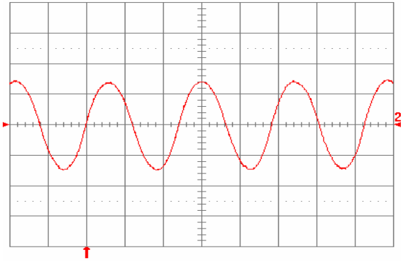
Fig. 2.5V.14: Input reflected ripple current, i_c (100 mA/div), measured at input terminals at full rated load current and V_{in} = 48 V. Refer to Fig. 2.5V.11 for test setup. Time scale: 1 \mu s/div.
