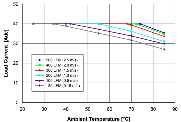
Fig. 1.2V.2: Available load current vs. ambient air temperature and airflow rates for QM48S40012 converter mounted horizontally with air flowing from pin 3 to pin 1, MOSFET temperature \leq 120^{\circ}\text{C} , V_{in} = 48\text{ V} .
