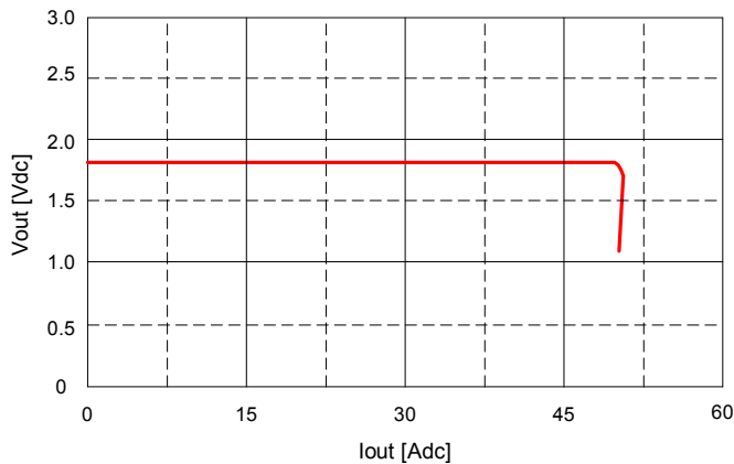
Fig. 1.8V.13: Output voltage vs. load current showing current limit point and converter shutdown point. Input voltage has almost no effect on current limit characteristic.
