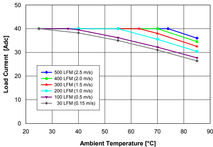
Fig. 1.5V.1: Available load current vs. ambient air temperature and airflow rates for QM48S40015 converter mounted vertically with air flowing from pin 3 to pin 1, MOSFET temperature \leq 120^{\circ}\text{C} , V_{in} = 48\text{ V} .
