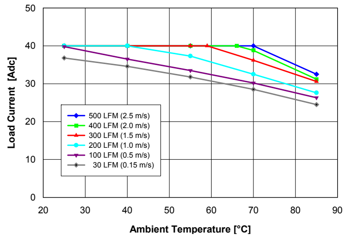
Fig. 2.0V.2: Available load current vs. ambient air temperature and airflow rates for QM48S40020 converter mounted horizontally with air flowing from pin 3 to pin 1, MOSFET temperature \leq 120^{\circ}\text{C} , V_{in} = 48\text{ V} .
