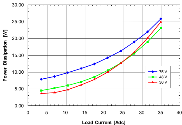
Fig. 25: Power dissipation vs. load current and input voltage for converter w/o baseplate mounted vertically with air flowing from pin 3 to pin 1 at a rate of 300 LFM (1.5 m/s) and T_a = 25^\circ\text{C} .
