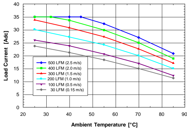
Fig. 3: Available output current vs. ambient air temperature and airflow rates for converter with baseplate mounted vertically with air flowing from pin 1 to pin 3, MOSFET temperature \leq 120^\circ\text{C} , V_{in} = 48\text{ V} .
