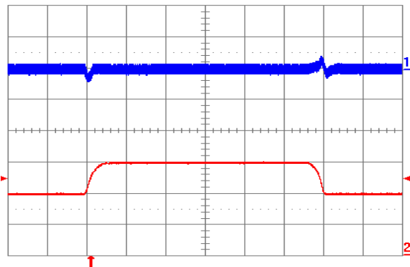
Fig. 9: Output voltage response to load current step-change (20 A – 30 A – 20 A) at V_{in} = 48\text{ V} . Top trace: output voltage (100 mV/div.). Bottom trace: load current (10 A/div.). Current slew rate: 0.1 A/ \mu\text{s} C_o = 1\text{ }\mu\text{F} ceramic. Time scale: 0.2 ms/div
