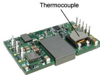
Fig. G: Location of the Thermocouple for Thermal Testing
