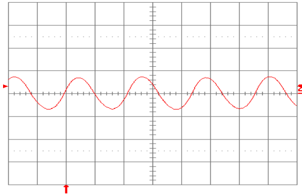
Fig. 13: Input reflected ripple current, i_c (500 mA/div.), measured at input terminals at full rated load current and V_{in} = 48 \text{ V} . Refer to Fig. 12 for test setup. Time scale: 1 \mu\text{s}/\text{div}
