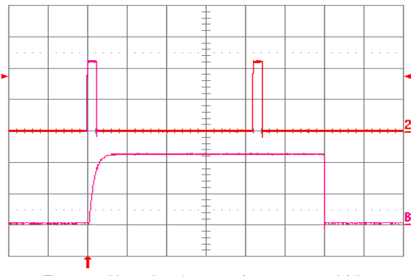
Figure 1.8V.24. Load current (top trace, 20 \text{ A}/\text{div} ., 50 \text{ ms}/\text{div} .) into a 10 \text{ m}\Omega short circuit during restart, at V_{in} = 48 \text{ V} . Bottom trace ( 20 \text{ A}/\text{div} ., 2 \text{ ms}/\text{div} .) is an expansion of the on-time portion of the top trace.
