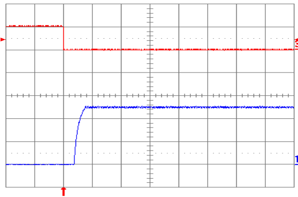
Figure 2.5V.15. Turn-on transient at full rated load current (resistive) with no output capacitor at V_{in} = 48\text{ V} , triggered via ON/OFF pin. Top trace: ON/OFF signal (5 V/div.). Bottom trace: output voltage (1 V/div.). Time scale: 2 ms/div.
