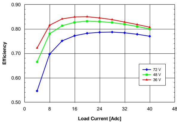
Figure 1.0V.11. Efficiency vs. load current and input voltage for QME48T40010 converter mounted horizontally with air flowing from pin 1 to pin 3 at a rate of 300 LFM (1.5 m/s) and T_a = 25^\circ\text{C} .
