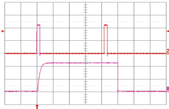
Figure 1.5V.24. Load current (top trace, 20 A/div., 50 ms/div.) into a 10 \text{ m}\Omega short circuit during restart, at V_{in} = 48 \text{ V} . Bottom trace (20 A/div., 2 ms/div.) is an expansion of the on-time portion of the top trace.
