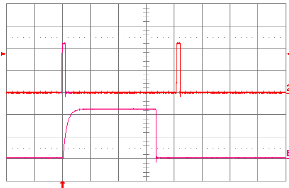
Figure 3.3V.24. Load current (top trace, 20 A/div., 50 ms/div.) into a 10 m \Omega short circuit during restart, at V_{in} = 48 \text{ V} . Bottom trace (20 A/div., 2 ms/div.) is an expansion of the on-time portion of the top trace.
