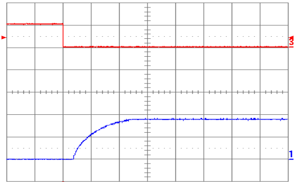
Figure 1.8V.16. Turn-on transient at full rated load current (resistive) plus 10,000 \mu\text{F} at V_{in} = 48\text{ V} , triggered via ON/OFF pin. Top trace: ON/OFF signal (5 V/div.). Bottom trace: output voltage (1 V/div.). Time scale: 2 ms/div.
