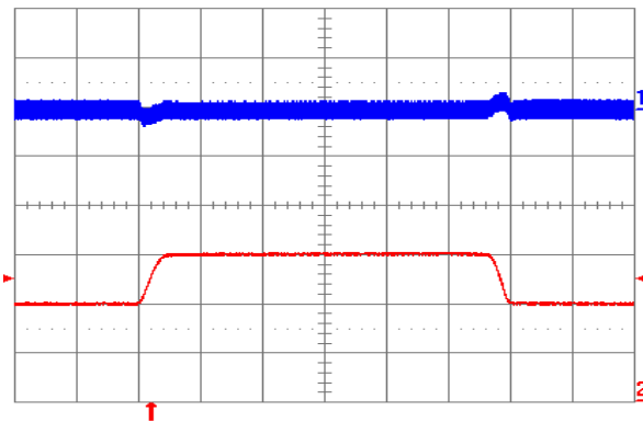
Figure 1.8V.17. Output voltage response to load current step-change (20 A – 30 A – 20 A) at V_{in} = 48\text{ V} . Top trace: output voltage (100 mV/div.). Bottom trace: load current (10 A/div.). Current slew rate: 0.1 A/ \mu\text{s} . C_o = 1\ \mu\text{F} ceramic. Time scale: 0.2 ms/div.
