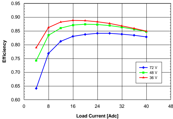
Figure 1.5V.11. Efficiency vs. load current and input voltage for QME48T40015 converter mounted horizontally with air flowing from pin 1 to pin 3 at a rate of 300 LFM (1.5 m/s) and T_a = 25\text{ }^{\circ}\text{C} .
