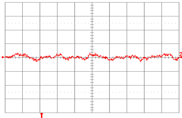
Figure 1.5V.22. Input reflected ripple current, i_s (10 mA/div.), measured through 10 \mu\text{H} at the source at full rated load current and V_{in} = 48 \text{ V} . Refer to Fig. 1.5V.20 for test setup. Time scale: 1 \mu\text{s}/\text{div} .
