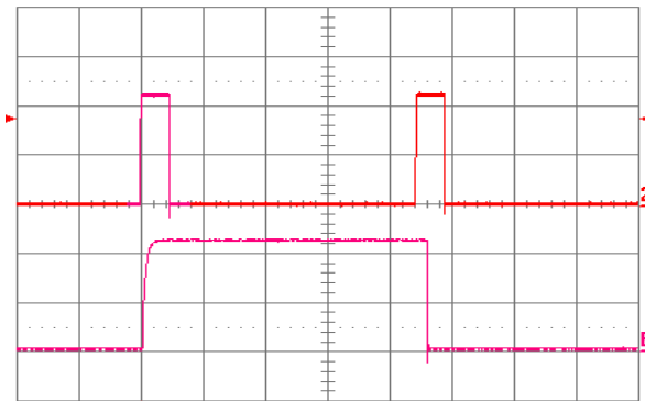
Figure 1.2V.24. Load current (top trace, 20 \text{ A}/\text{div} ., 50 \text{ ms}/\text{div} .) into a 10 \text{ m}\Omega short circuit during restart, at V_{in} = 48 \text{ V} . Bottom trace ( 20 \text{ A}/\text{div} ., 5 \text{ ms}/\text{div} .) is an expansion of the on-time portion of the top trace.
