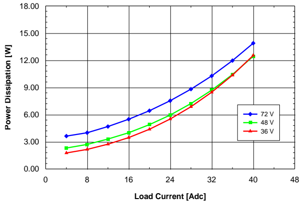
Figure 2.5V.13. Power dissipation vs. load current and input voltage for QME48T40025 converter mounted horizontally with air flowing from pin 1 to pin 3 at a rate of 300 LFM (1.5 m/s) and T_a = 25\text{ }^\circ\text{C} .
