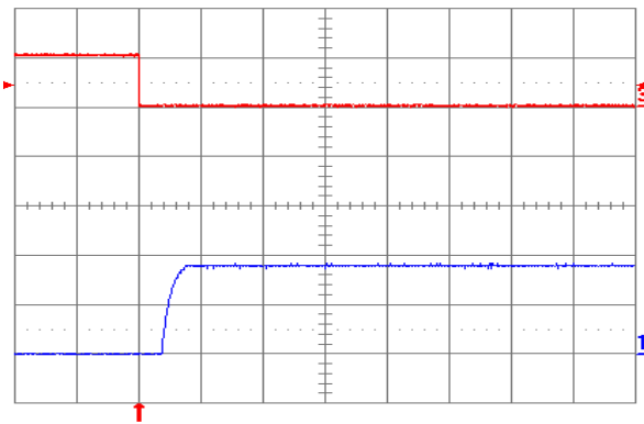
Figure 1.8V.15. Turn-on transient at full rated load current (resistive) with no output capacitor at V_{in} = 48\text{ V} , triggered via ON/OFF pin. Top trace: ON/OFF signal (5 V/div.). Bottom trace: output voltage (1 V/div.). Time scale: 2 ms/div.
