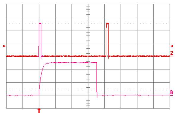
Fig. 16: Load current (top trace, 20 \text{ A}/\text{div} ., 50 \text{ ms}/\text{div} .) into a 10 \text{ m}\Omega short circuit during restart, at V_{in} = 48 \text{ V} . Bottom trace ( 20 \text{ A}/\text{div} ., 2 \text{ ms}/\text{div} .) is an expansion of the on-time portion of the top trace.
