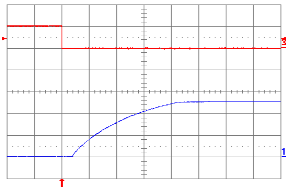
Fig. 8: Turn-on transient at full rated load current (resistive) plus 10,000 µF at V_{in} = 48\text{ V} , triggered via ON/OFF pin. Top trace: ON/OFF signal (5 V/div.). Bottom trace: output voltage (5 V/div.). Time scale: 2 ms/div.
