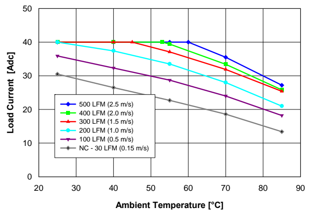
Fig. 2 : Available load current vs. ambient air temperature and airflow rates for converter with G height pins mounted horizontally with air flowing from pin 1 to pin 3, MOSFET temperature \leq 120^\circ\text{C} , V_{in} = 48\text{ V} .
