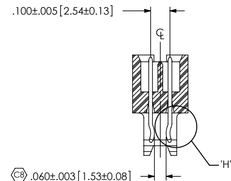
SECTION "G"-"G" SCALE 2 : 1
