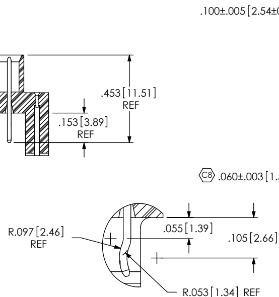
DETAIL 'H' SCALE 4 : 1
