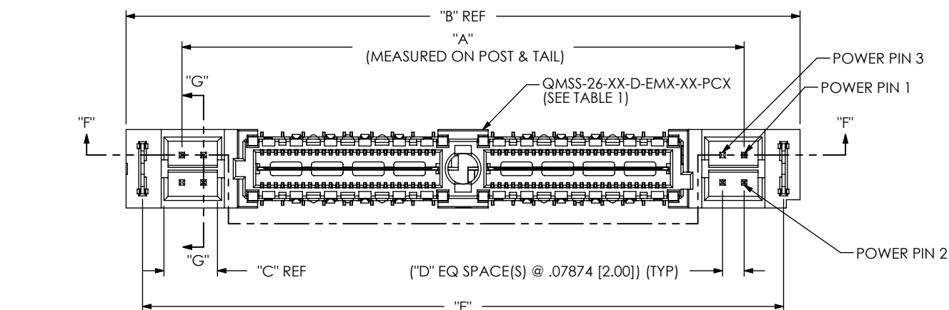
FIG 2 -PCX OPTION QMSS-032-01-X-D-DP-EM2-PC4 SHOWN [DIFFERENT AS SHOWN, OTHERWISE SAME AS FIG 1] [AVAILABLE ON -016, -032 & -048 POSITIONS ONLY]
