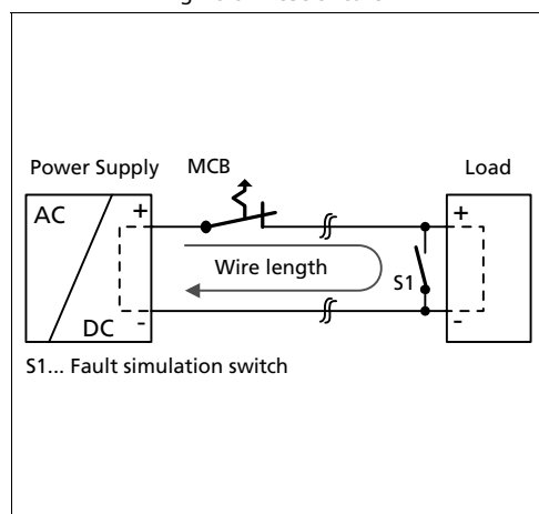
Fig. 25-5 Test circuit
