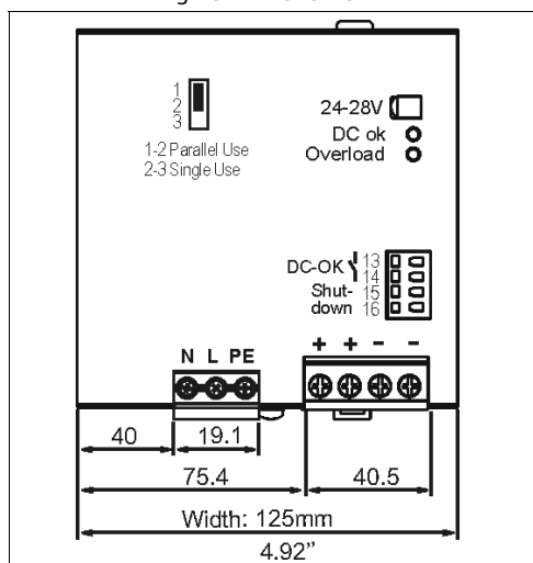
Fig. 23-1 Front view
