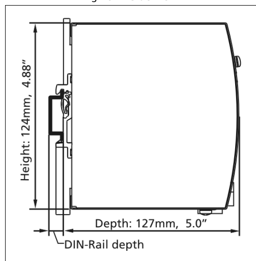
Fig. 23-2 Side view
