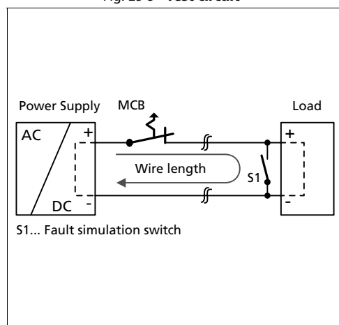
Fig. 25-5 Test circuit
