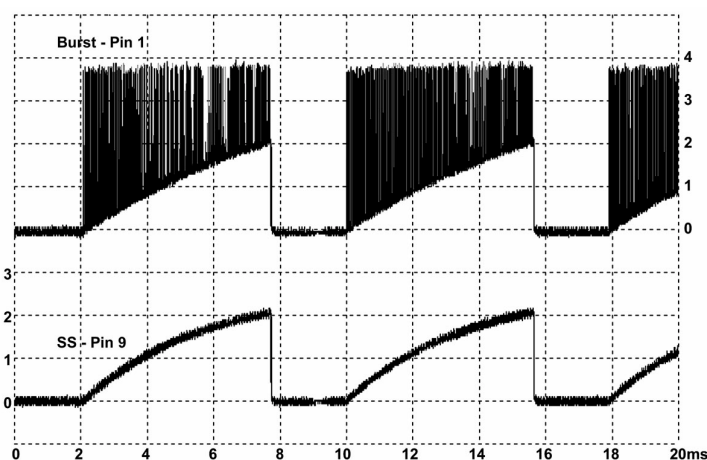
Figure 3.1 Spread-Spectrum Waveforms
