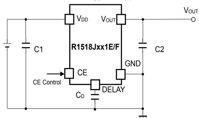
R1518xxxE/F Typical Application
