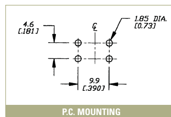
P.C. MOUNTING
