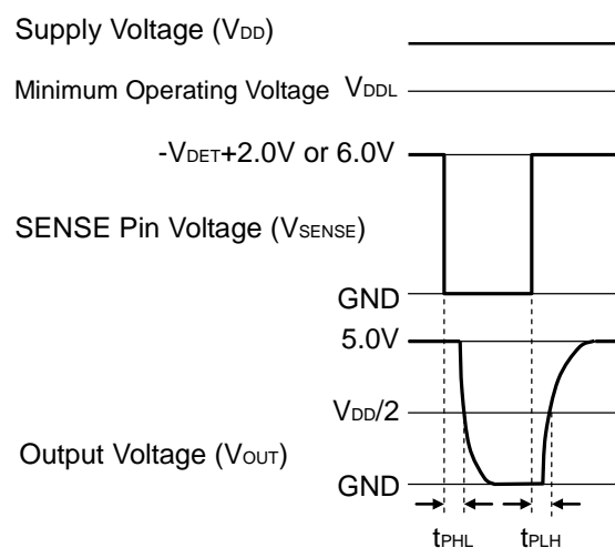
CMOS Output (R3117xxx2C)
