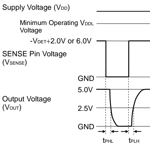
Nch Open Drain Output (R3117xxx1A)
