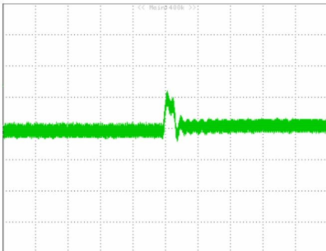
Figure 8: Output voltage response to step-change in load current (75%-50% of I_o , max; di/dt = 0.1A/\mu S ). Load cap: 10 \mu F Low ESR capacitor and 1 \mu F ceramic capacitor. Top Trace: V_{out} (50mV/div), Scope measurement should be made using a BNC cable (length shorter than 20 inches). Position the load between 51 mm to 76 mm (2 inches to 3 inches) from the module.
