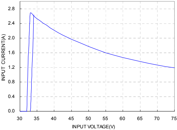
Figure 3: Typical input characteristics at room temperature
