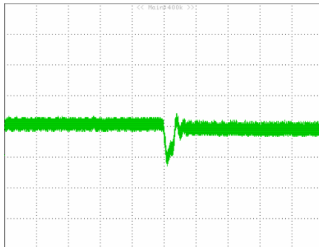
Figure 9: Output voltage response to step-change in load current (50%-75% of I_o , max; di/dt = 0.1A/\mu S ). Load cap: 10 \mu F Low ESR capacitor and 1 \mu F ceramic capacitor. Top Trace: V_{out} (50mV/div), Scope measurement should be made using a BNC cable (length shorter than 20 inches). Position the load between 51 mm to 76 mm (2 inches to 3 inches) from the module.
