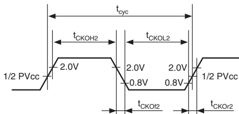
Figure 37.2 (2) CKIO Clock Output Timing 2
