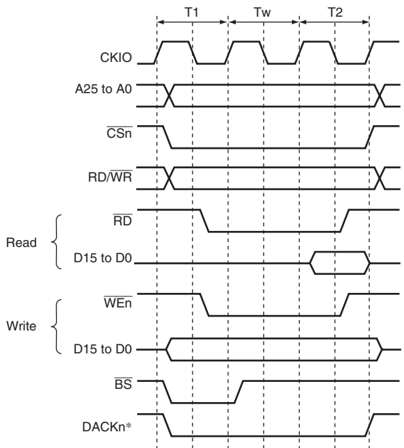
Figure 9.7 Wait Timing for Normal Space Access (Software Wait Only)
