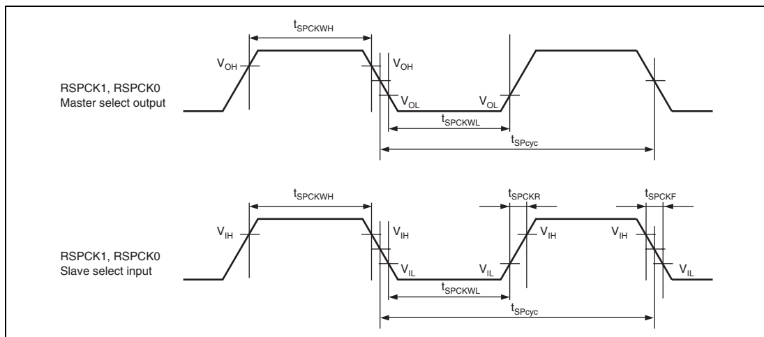
Figure 37.45 Clock Timing
