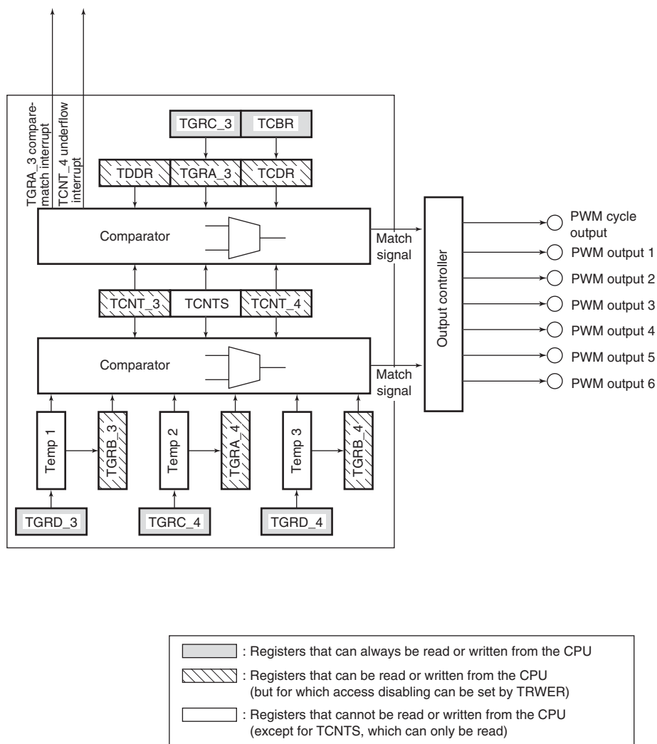
Figure 11.37 Block Diagram of Channels 3 and 4 in Complementary PWM Mode
