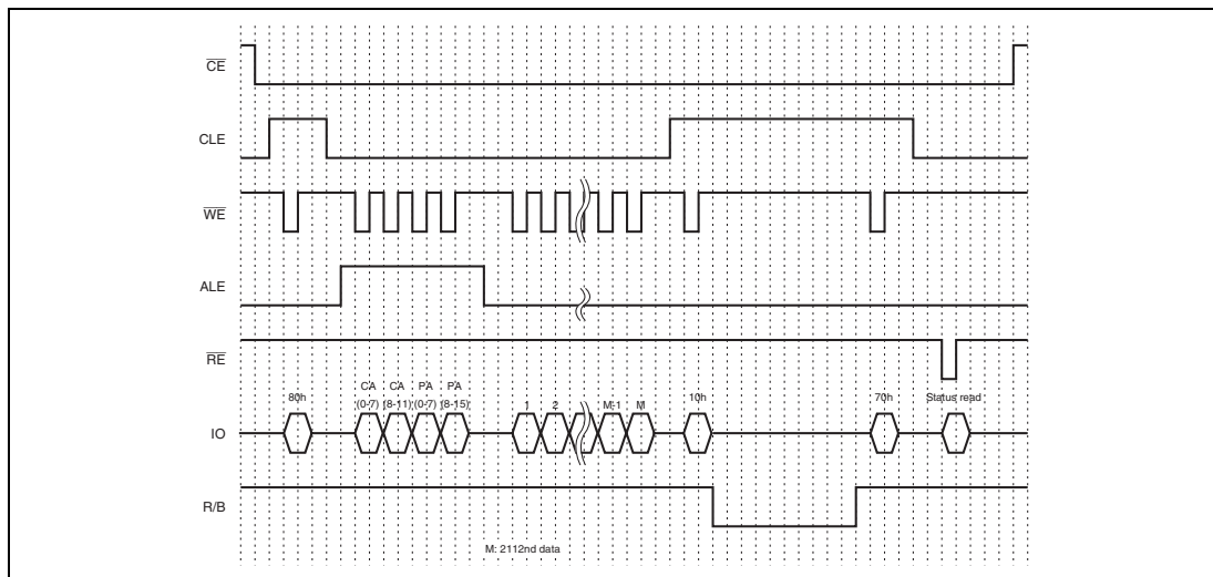
Figure 26.13 Programming Operation Timing for NAND-Type Flash Memory
