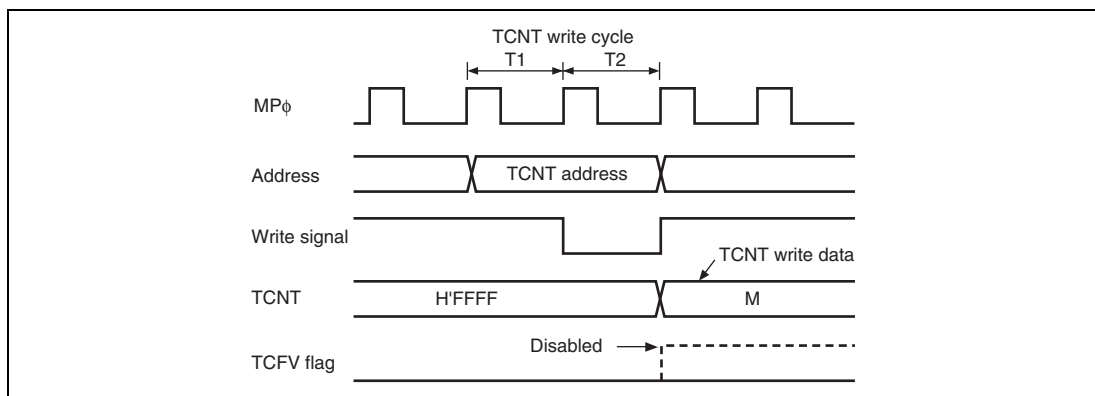
Figure 11.112 Contention between TCNT Write and Overflow
