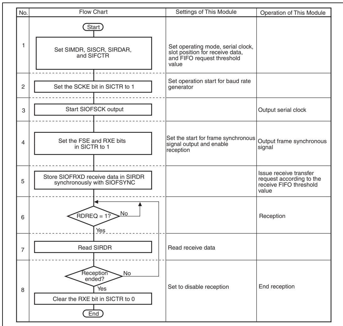
Figure 20.7 Example of Receive Operation in Master Mode
