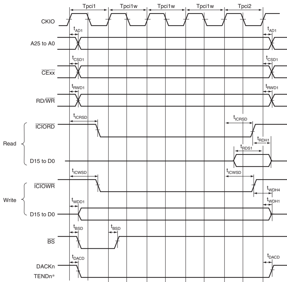
Figure 37.36 PCMCIA I/O Card Bus Cycle (TED = 0 Cycle, TEH = 0 Cycle, No Wait)
