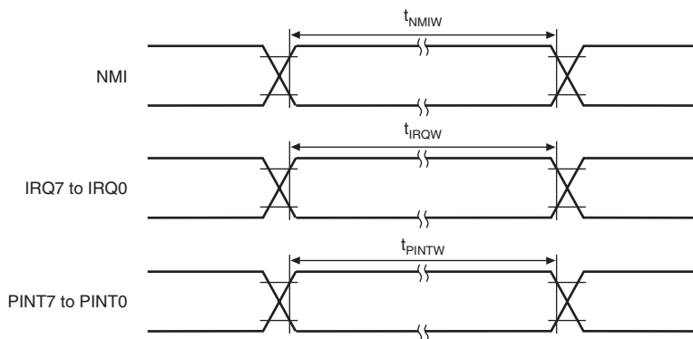
Figure 37.7 (2) Interrupt Signal Input Timing
