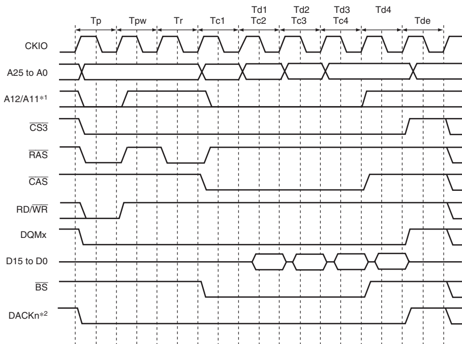
Figure 9.21 Burst Read Timing (Bank Active, Different Row Addresses in the Same Bank, CAS Latency 1)
