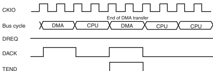
Figure 10.15 Example of DMA Transfer End Signal Timing (Cycle Steal Mode Level Detection)
