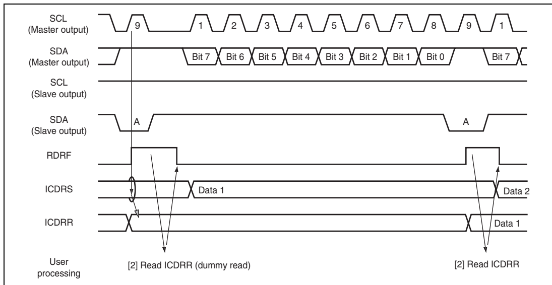
Figure 18.11 Slave Receive Mode Operation Timing (1)
