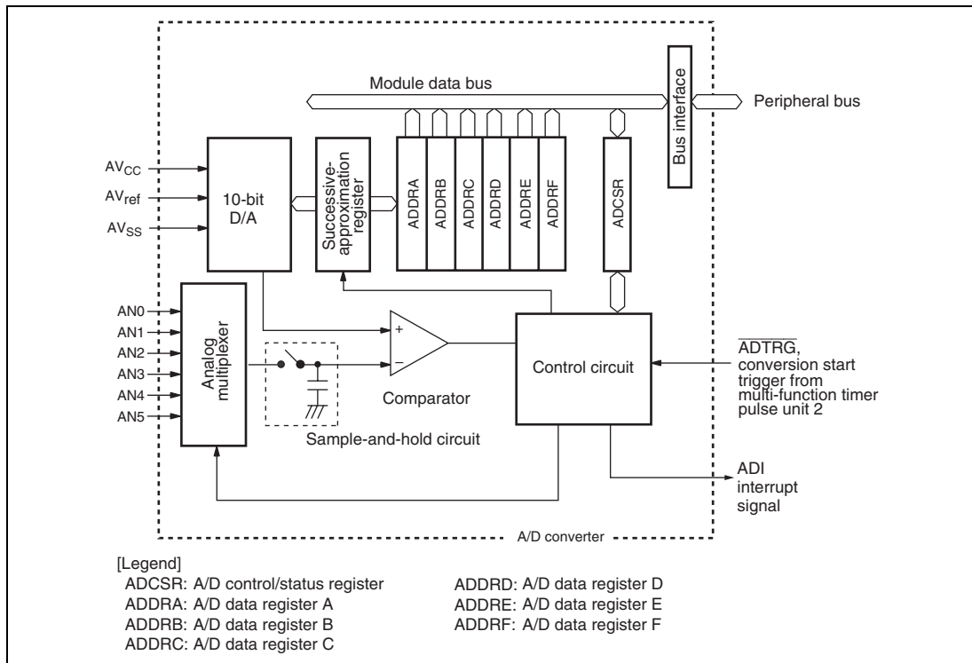
Figure 25.1 Block Diagram of A/D Converter
