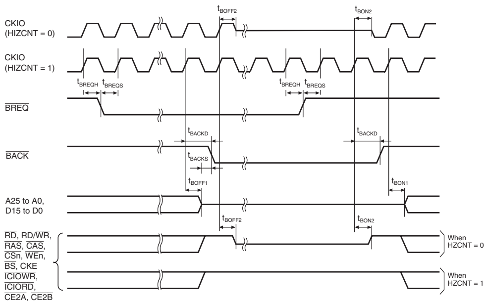
Figure 37.8 Bus Release Timing
