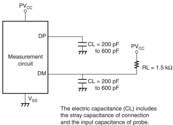
Figure 37.67 Measurement Circuit (Low-Speed)
