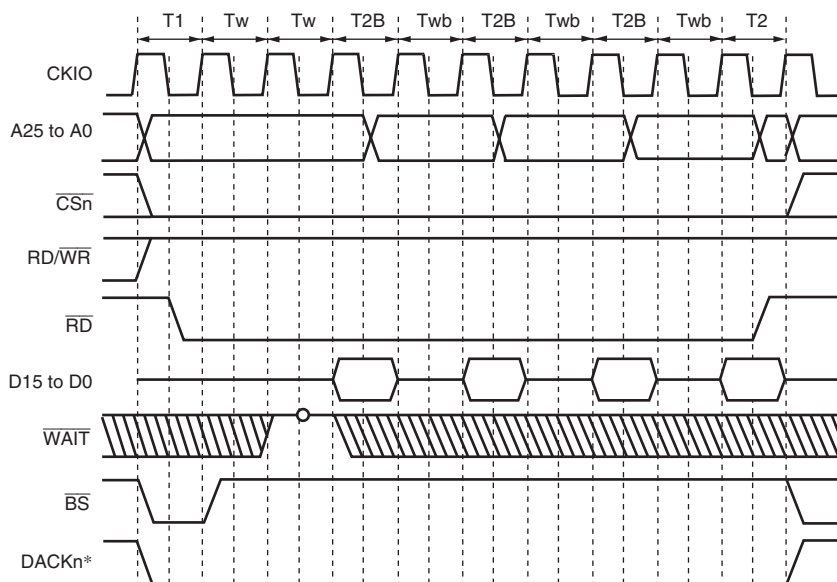
Figure 9.31 Burst ROM Access Timing (Clocked Asynchronous) (Bus Width = 16Bits, 16-Byte Transfer (Number of Burst 4-4), Wait Cycles Inserted in First Access = 2, Wait Cycles Inserted in Second and Subsequent Access Cycles = 1)
