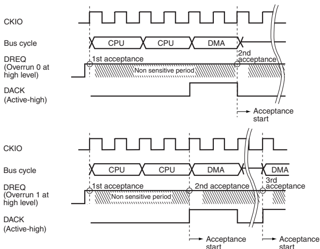
Figure 10.14 Example of DREQ Input Detection in Burst Mode Level Detection
