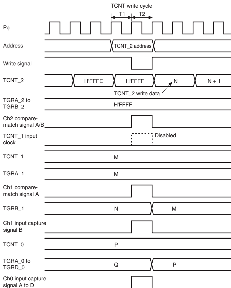
Figure 11.107 TCNT_2 Write and Overflow/Underflow Contention with Cascade Connection
