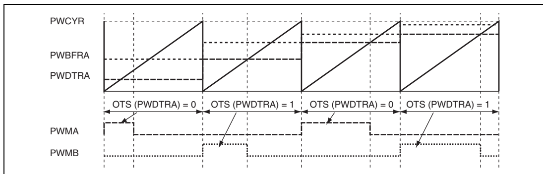
Figure 35.7 PWM Operation
