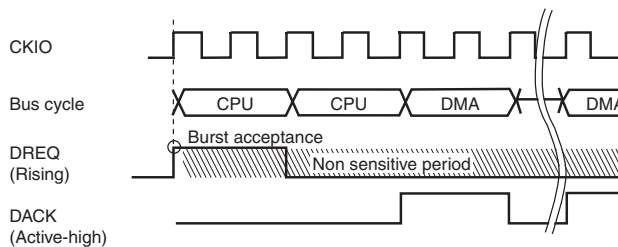
Figure 10.13 Example of DREQ Input Detection in Burst Mode Edge Detection
