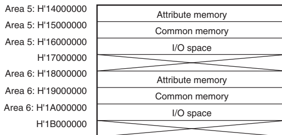
Figure 9.39 Example of PCMCIA Space Allocation (CS5WCR.SA[1:0] = B'10, CS6WCR.SA[1:0] = B'10)
