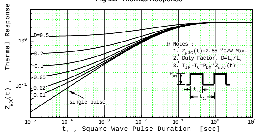
Fig 11. Thermal Response
