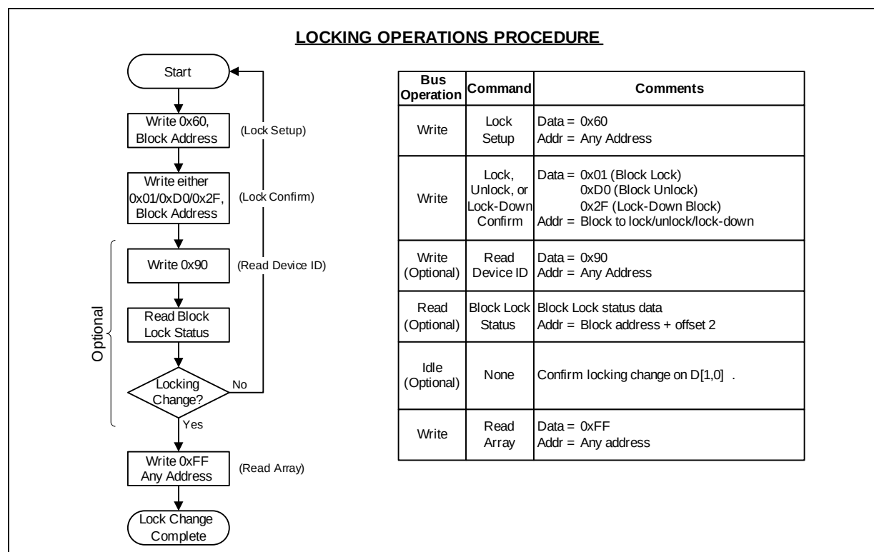
Figure 21: Locking Operations Flowchart
