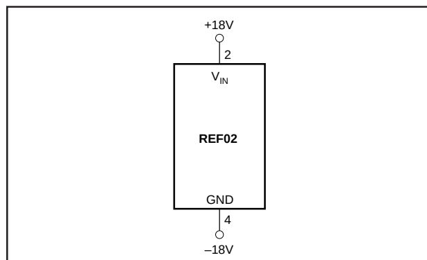
FIGURE 1. Burn-In Circuit.
