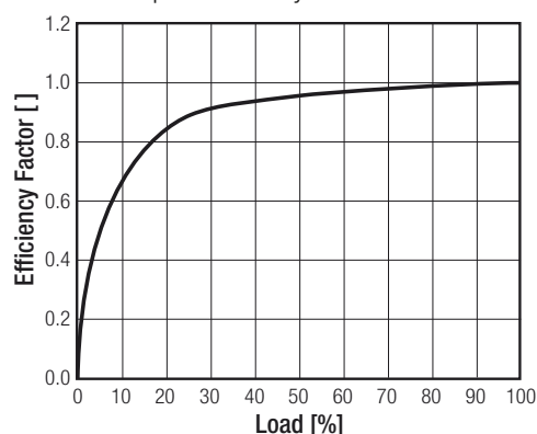
Graph1: Efficiency Factor vs. Load
