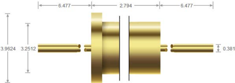
RF/50 Ohm, Flanged Body (mm)
