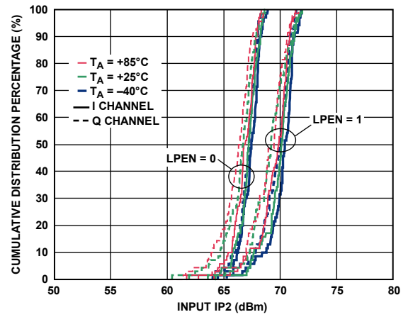
Figure 30. Input IP2
