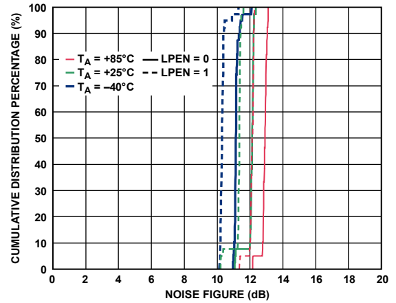
Figure 31. Noise Figure
