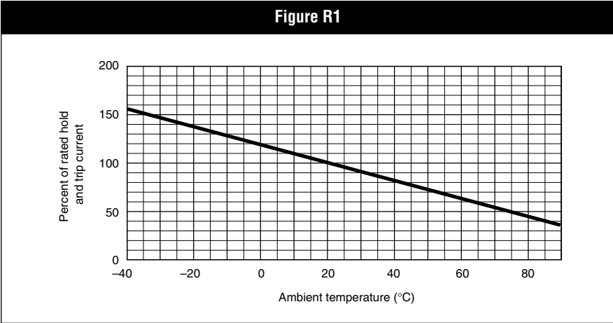
Figures R1–R4. Thermal Derating Curves for Radial-led Devices
