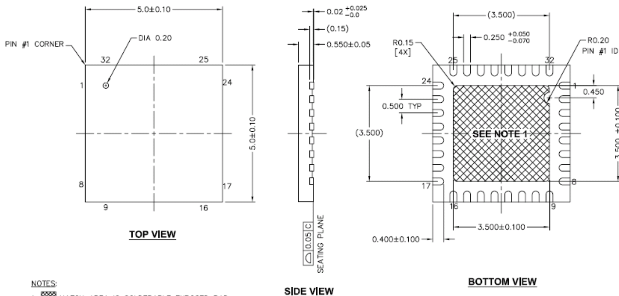
Figure 19. 32-Pin (5 x 5 x 0.6 mm) QFN
