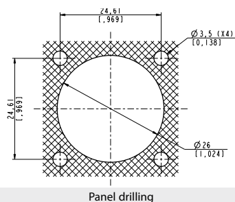
Panel drilling
